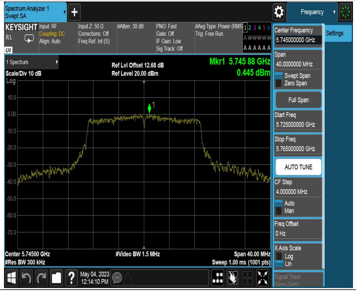
11N20SISO_Ant0_5745
