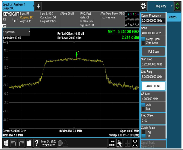
11AC20SISO_Ant0_5240
