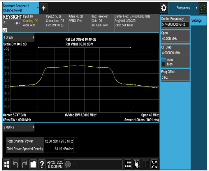
11AC20SISO_Ant2_5745
