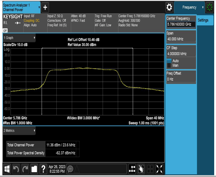
11AC20SISO_Ant1_5785
