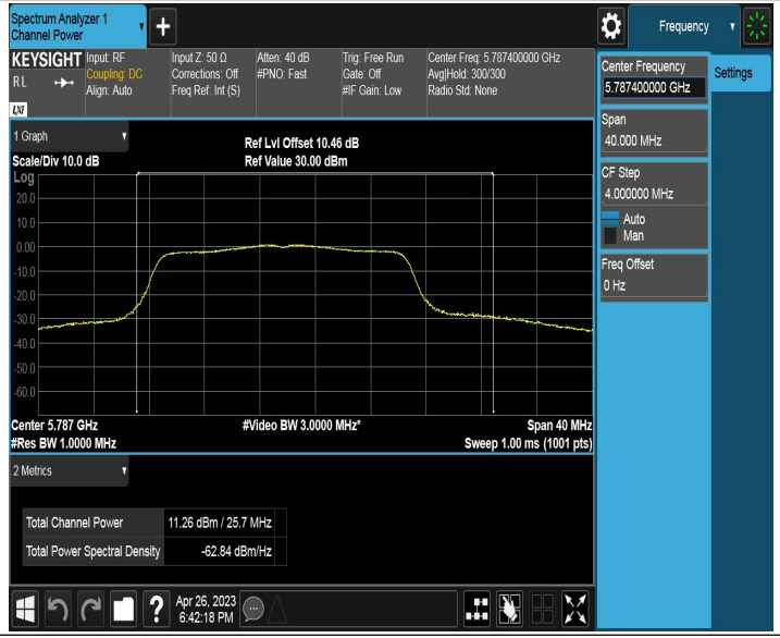
11N20SISO_Ant1_5785
