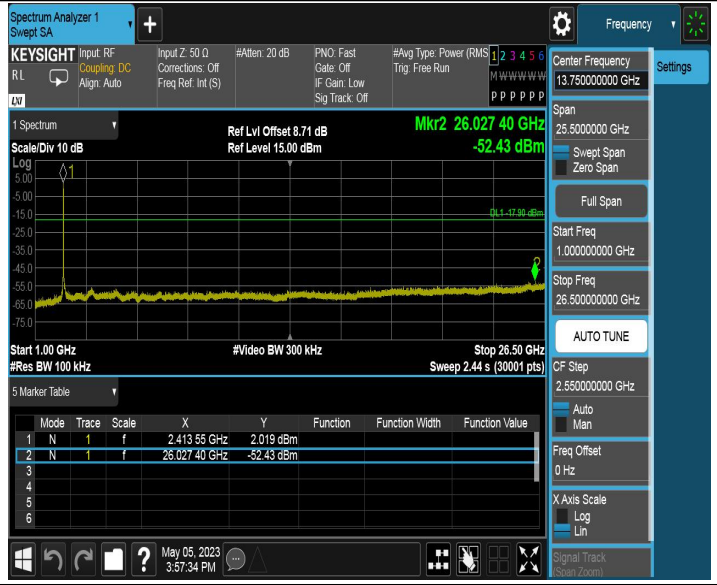
11N20SISO_Ant2_2412_0~Reference
