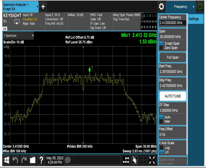
11N20SISO_Ant2_2412_0~Reference
