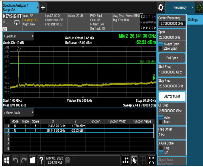
11G_Ant2_2462_0~Reference
