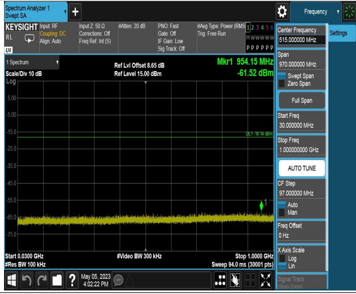
11N20SISO_Ant1_2462_30~1000
