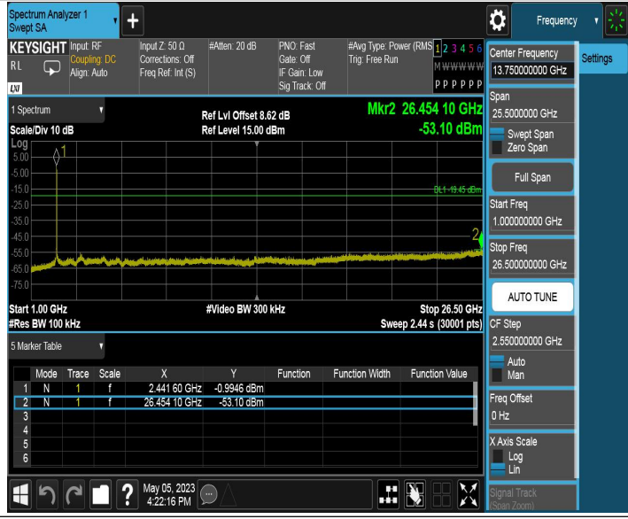
11G_Ant2_2437_1000~26500
