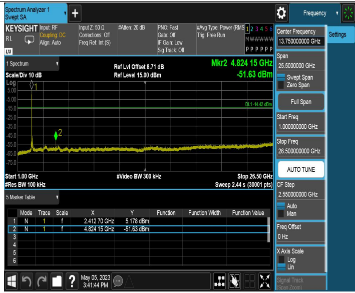
11B_Ant2_2412_0~Reference
