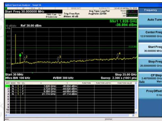
Spurious emission
