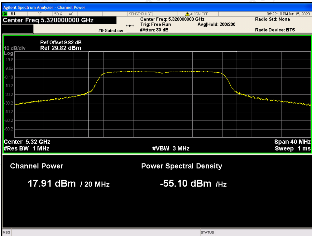
Power NVNT 802.11a 5500MHz Ant2
