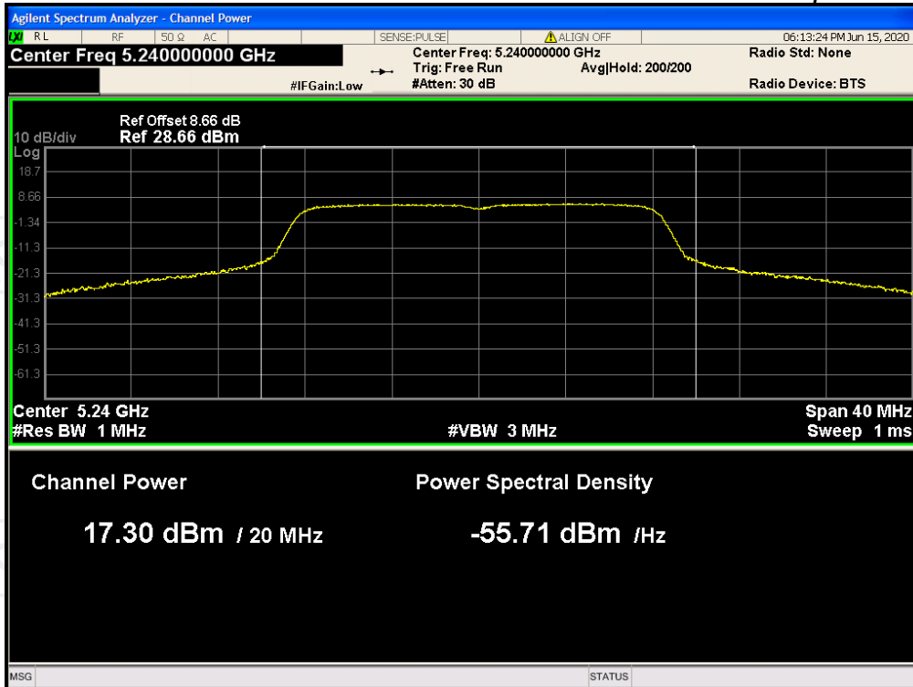
Power NVNT 802.11a 5260MHz Ant2
