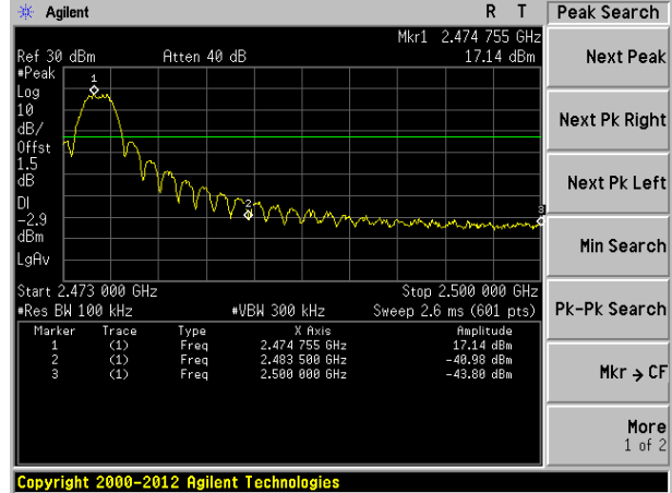
Highest channel(2475MHz)
