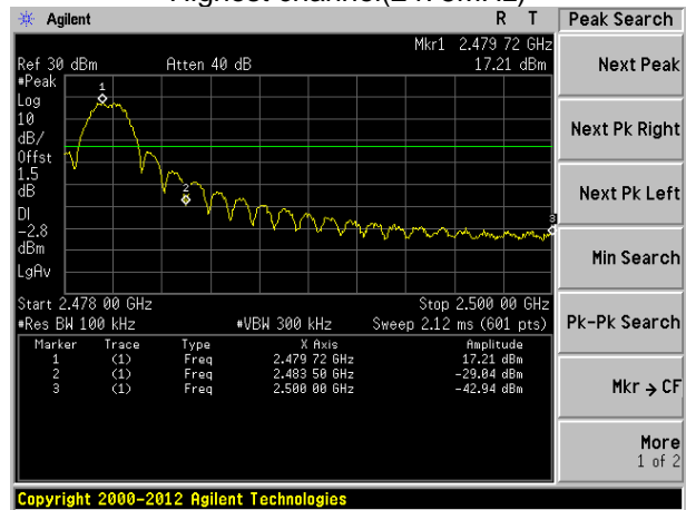
Highest channel(2480MHz)
