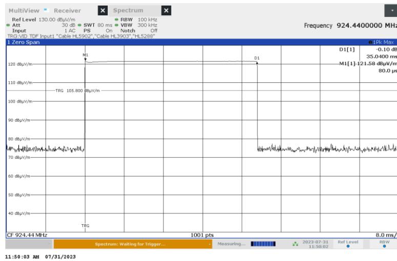
Plot 7.6.11 Transmission pulse period
