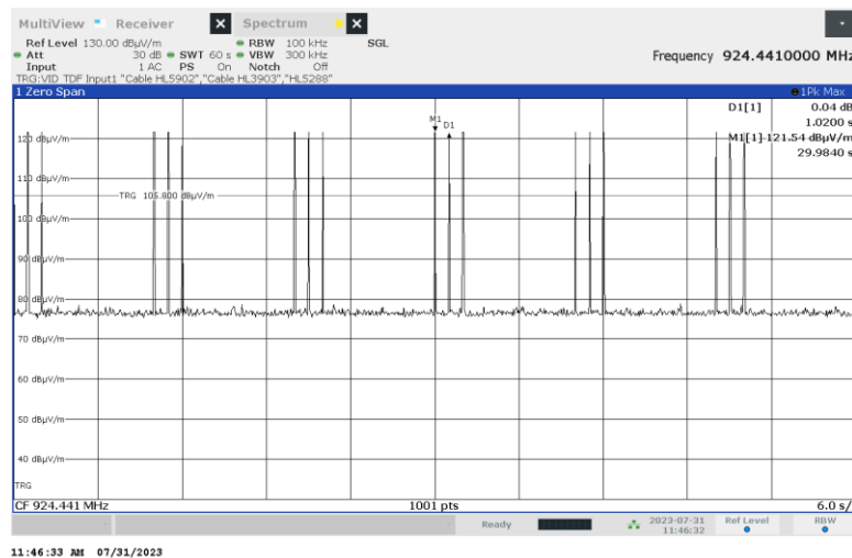
Plot 7.6.11 Transmission pulse period
