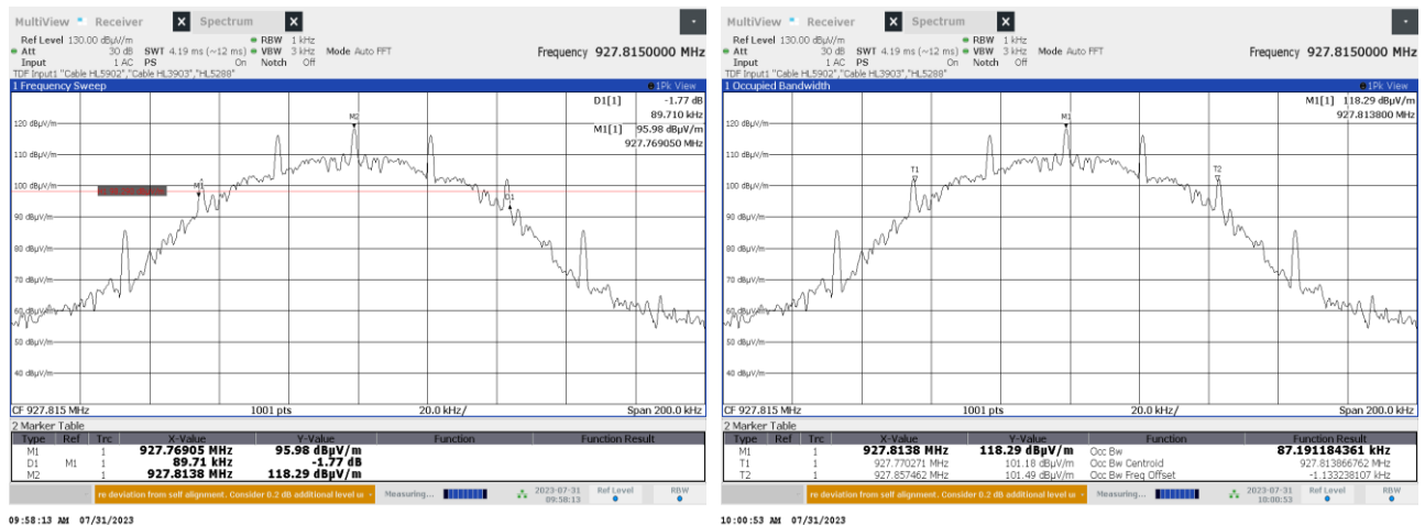
Plot 7.1.3 The 20 dB bandwidth test result at high frequency
