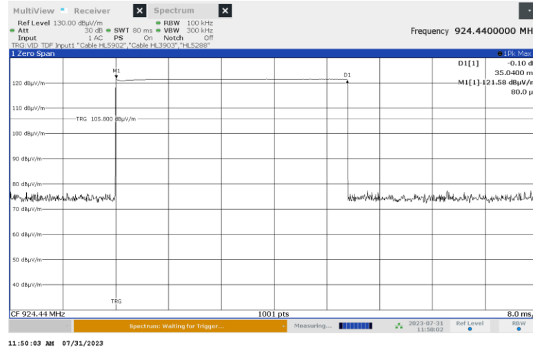
Plot 7.4.2 Single transmission period
