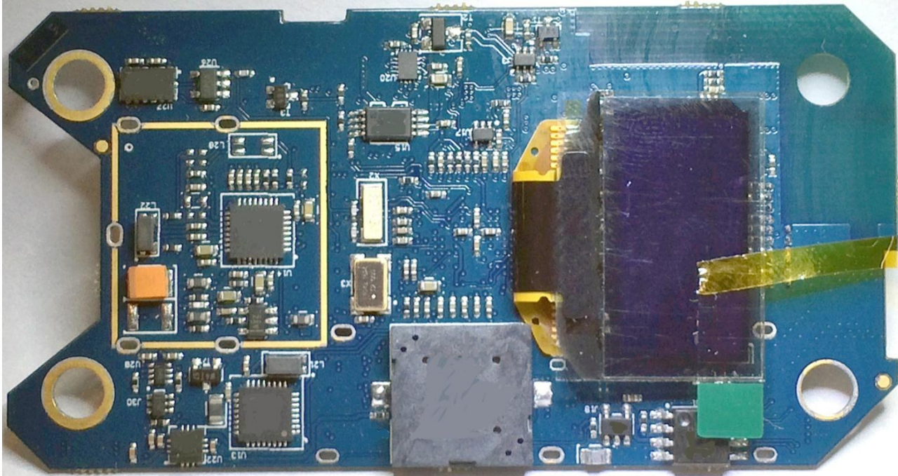
PCB WITH OLED SCREEN - FRONT
