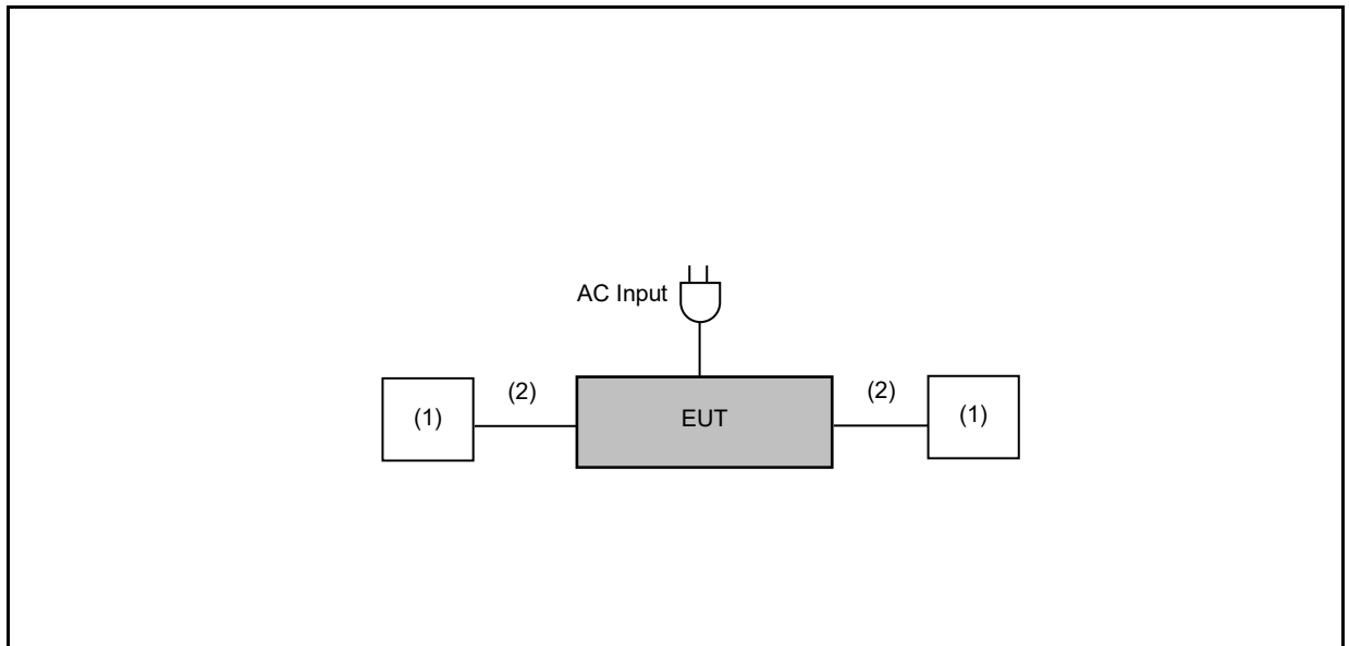
Conduction Emission
