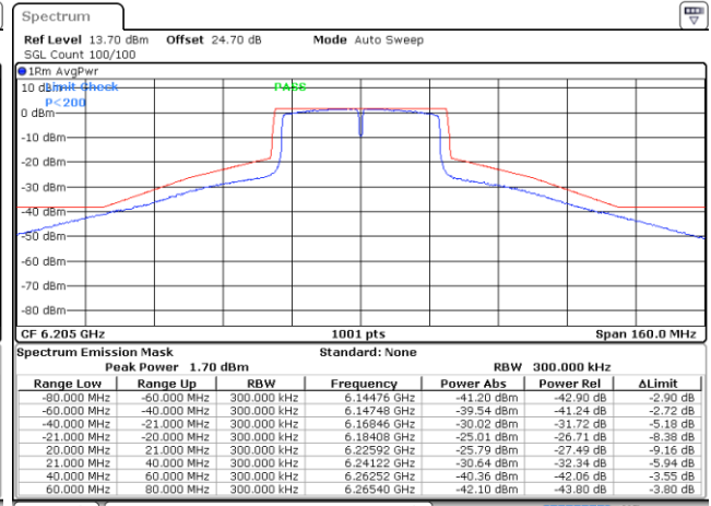
Plot on Channel 6205MHz
