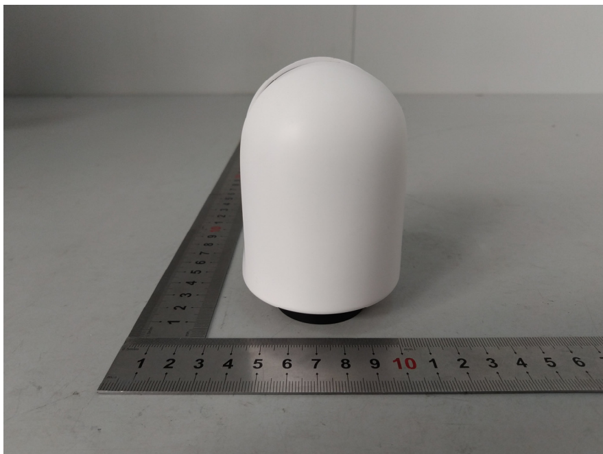
EUT (Speed 6S) – Left View
