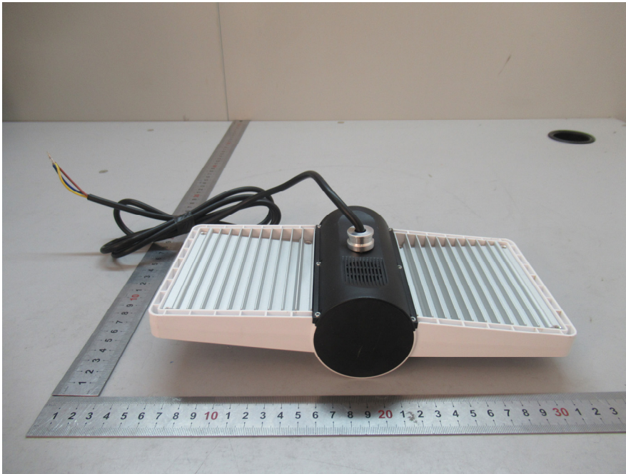
EUT (Flight 1S) – Rear View
