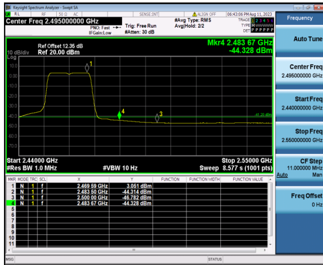
11N20SISO_Ant1_High_2462_AV
