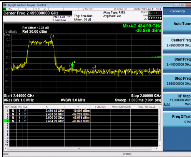
11N20SISO_Ant1_High_2462_Peak
