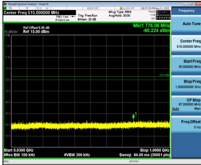
11N20SISO_Ant1_2437_30~1000
