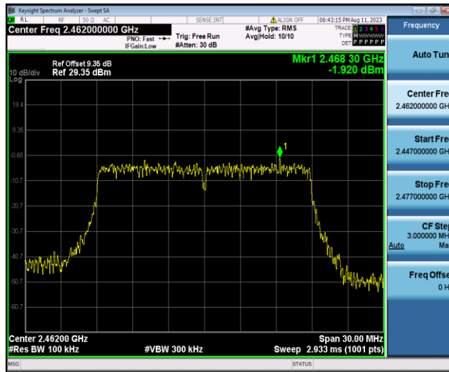
11N20SISO_Ant1_2462_0~Reference
