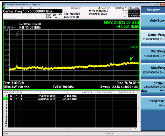
11N20SISO_Ant1_2437_1000~26500
