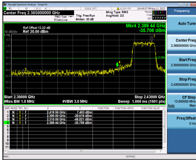
11N20SISO_Ant1_Low_2412_Peak
