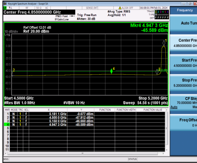
11A_Ant1_Low_5180_Peak
