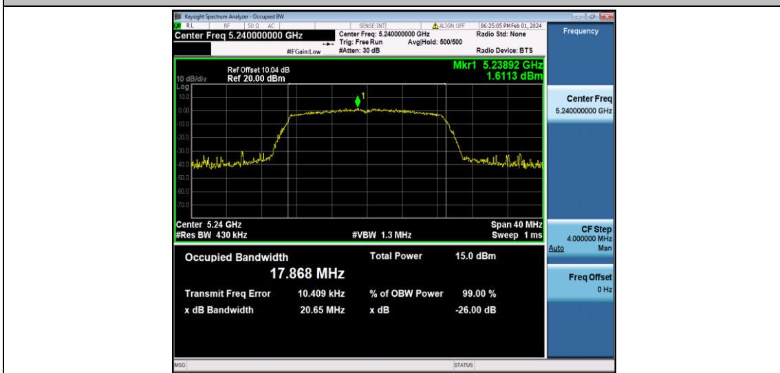
11N20SISO_Ant1_5240
