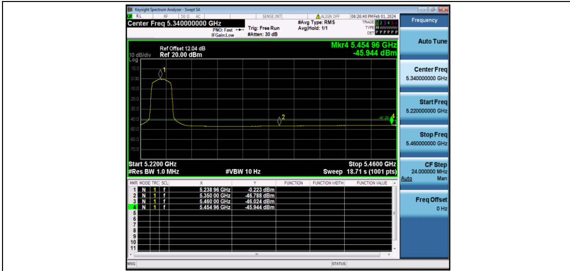
11N20SISO_Ant1_High_5240_Peak
