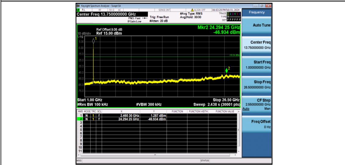
11N20SISO_Ant1_2462_1000~26500
