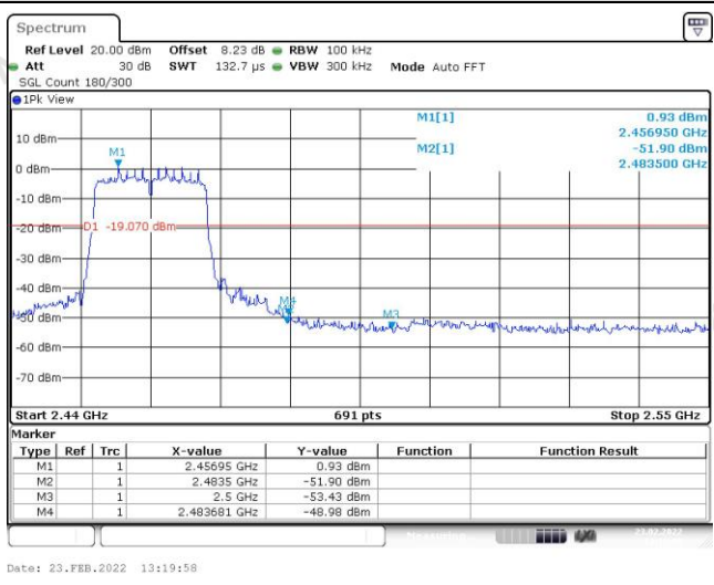
Right bandedge
