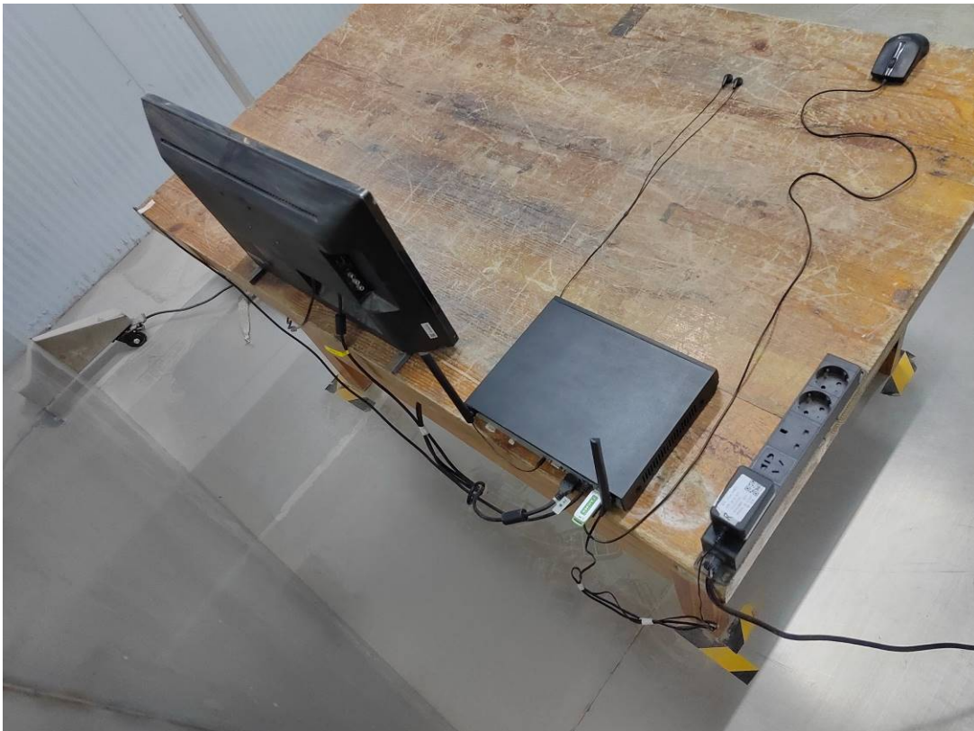
Conducted Emissions Side View - HDMI output
