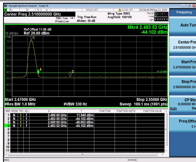
BLE_Ant1_High_2480_Peak
