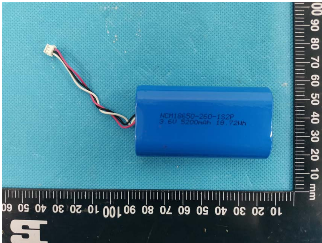
Battery 2
