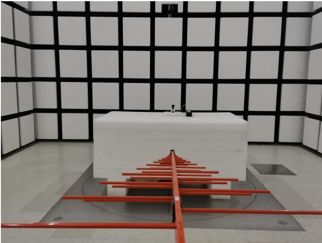
Radiated Emission Below 1GHz View AC
