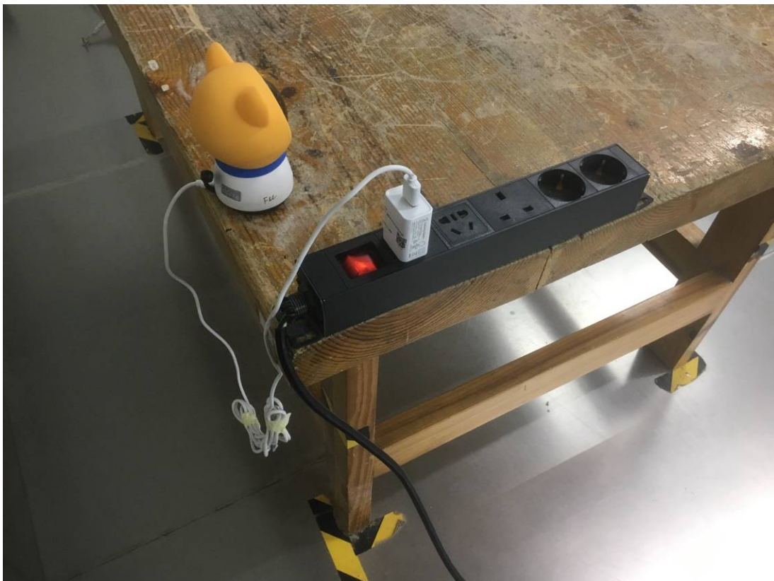
Conducted Emissions Side View #2 Adapter
