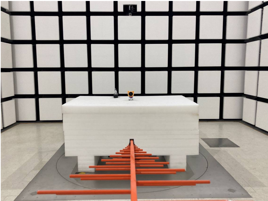
Radiated Emission Below 1GHz View #2 Adapter
