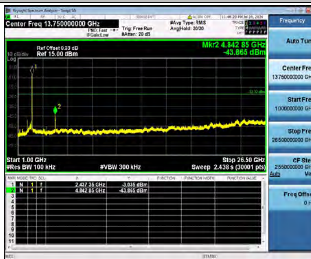
11AX40SISO_Ant1_2437_0~Reference
