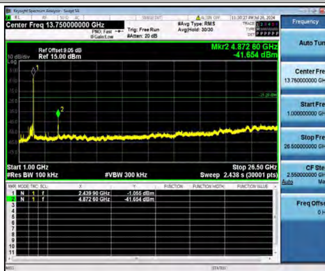
11N40SISO_Ant1_2452_0~Reference
