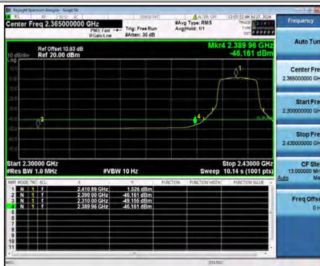
11AX20SISO_Ant1_Low_2412_Peak
