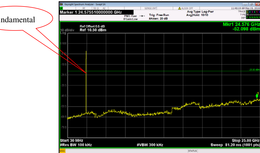
Middle Channel
