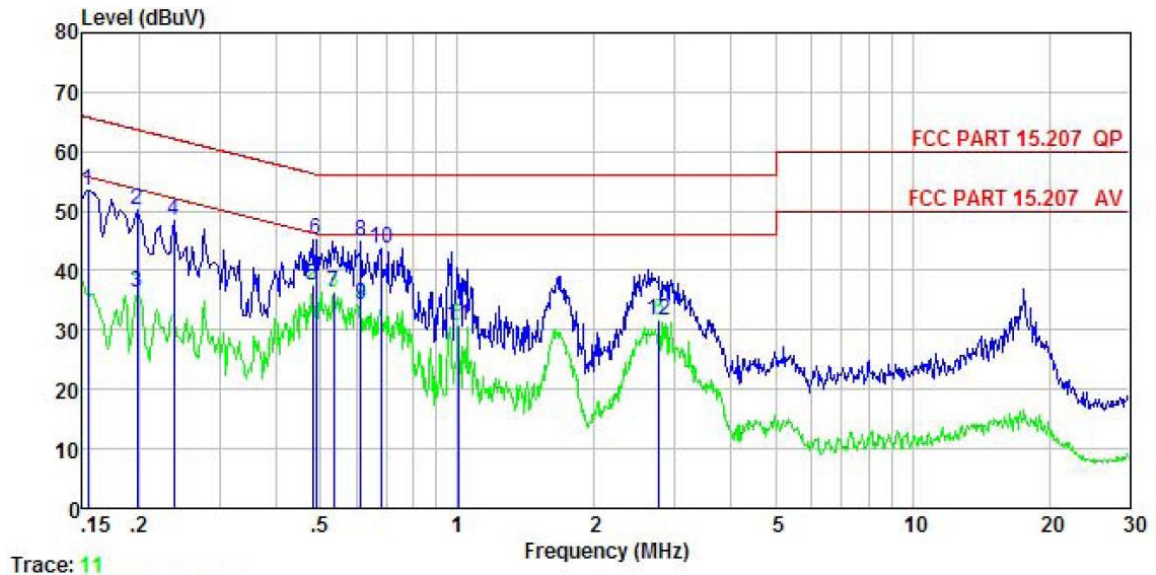
Trace: 11
