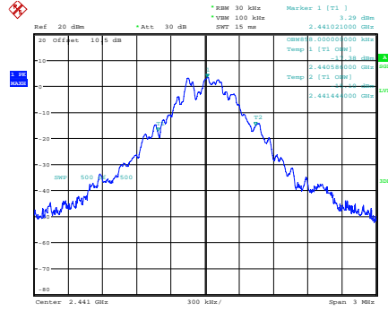
GFSK_Middle
