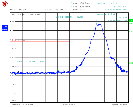
GFSK_Low
