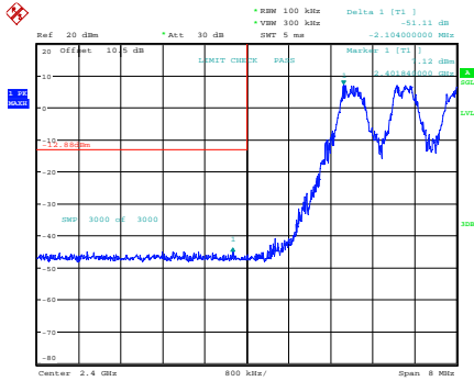
GFSK_Hopping_Lower
