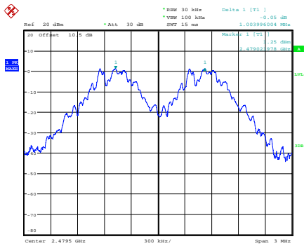
GFSK_High
