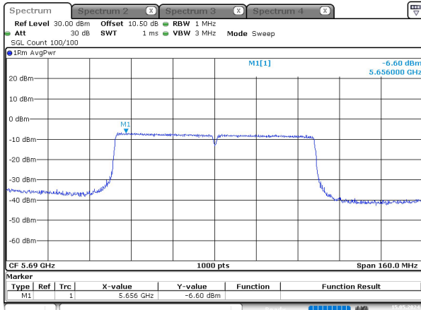
ac80_5690MHz_Chain 0
