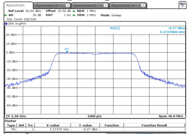
n20_5580MHz_Chain 0
