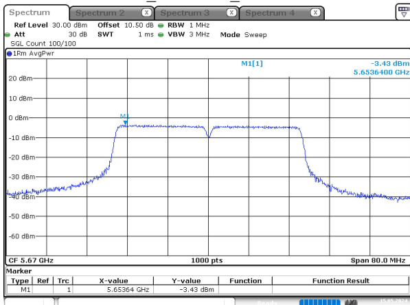
n40_5670MHz_Chain 0
