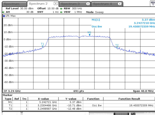
a_5240MHz_Chain 0
