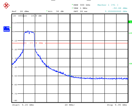
n20_5180MHz_Chain 0
