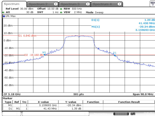
a_ 5180 MHz_Chain 0
