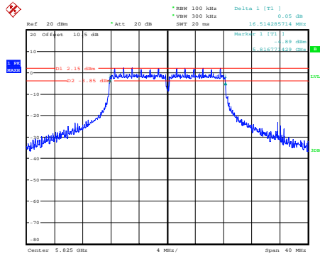
a_5825MHz_Chain 0
