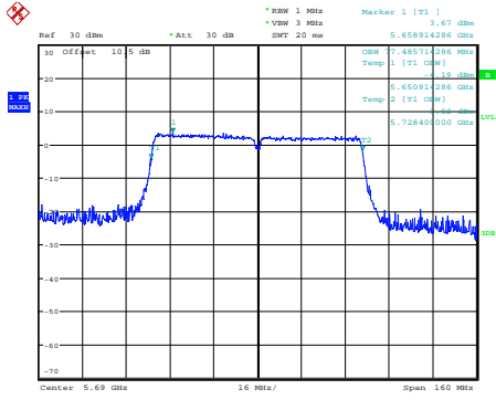
ac80_5690MHz_Chain 0
