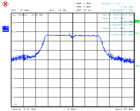
n40_5670MHz_Chain 0
