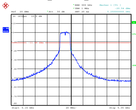
a_5240MHz_Chain 0
