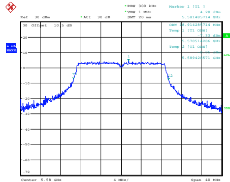
n20_5580MHz_Chain 0
