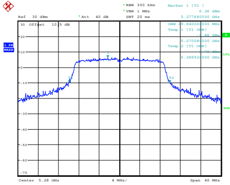
n20_5280MHz_Chain 0
