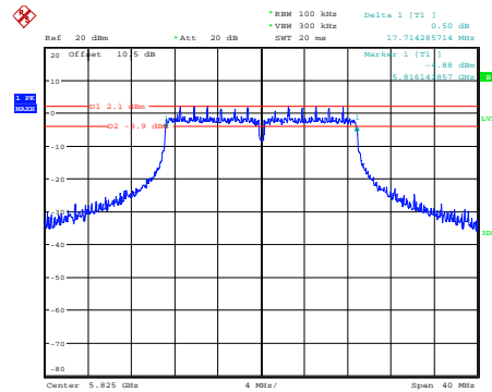
n20_5825MHz_Chain 0
