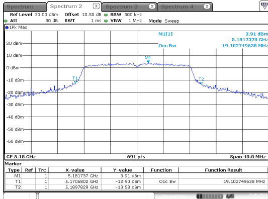
a_5180MHz_Chain 0
