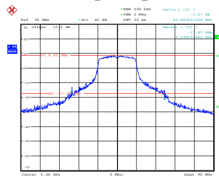
n20_5260MHz_Chain 0
