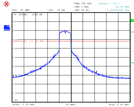
ax20_5240MHz_Chain 0
