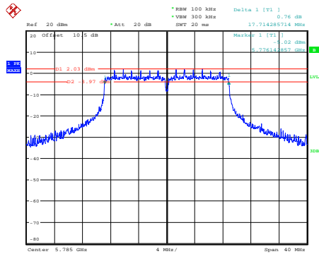
n20_5785MHz_Chain 0
