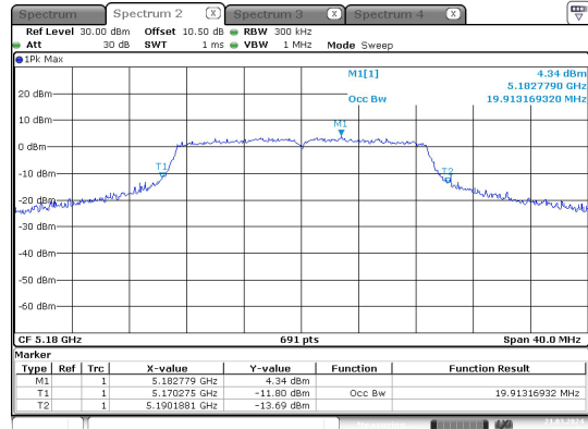
n20_5180MHz_Chain 0
