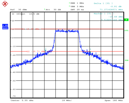
ax40_5550MHz_Chain 0
