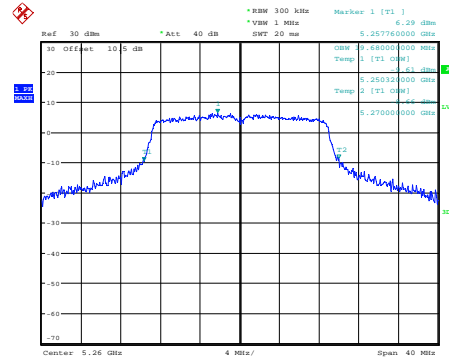
n20_5260MHz_Chain 0
