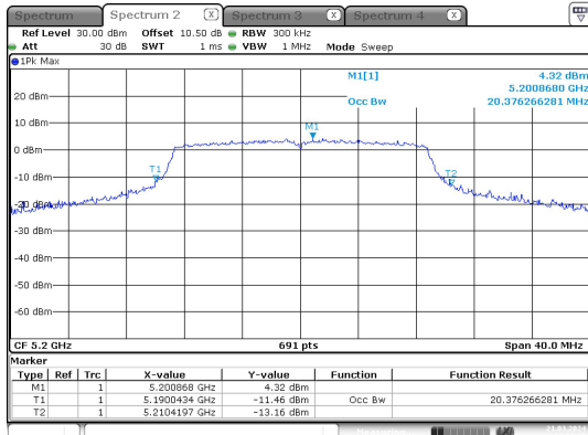
n20_5200MHz_Chain 0
