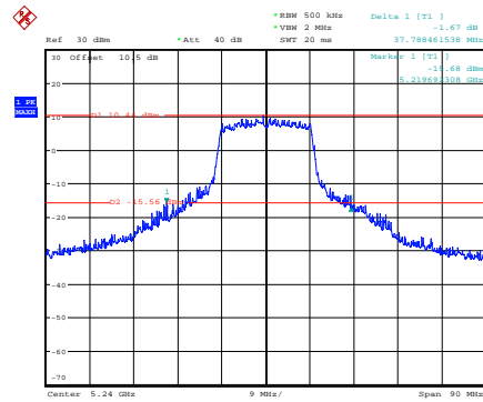
ax20_5240MHz_Chain 0
