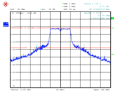
n40_5550MHz_Chain 0
