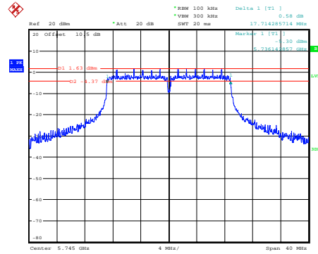
n20_5745MHz_Chain 0
