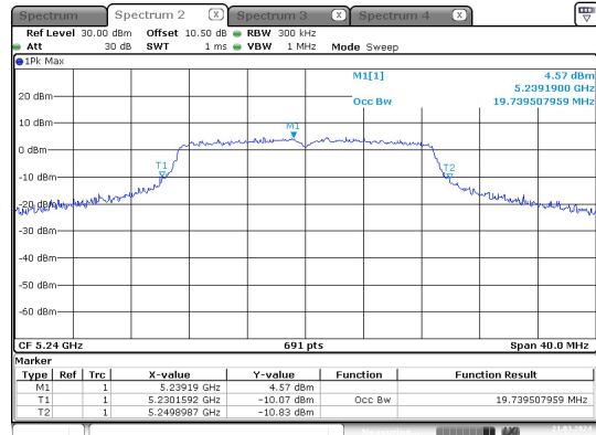
n20_5240MHz_Chain 0
