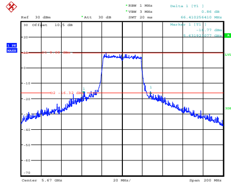
ax40_5670MHz_Chain 0
