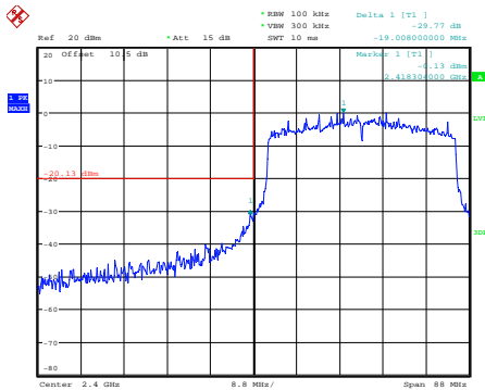
ax40_2422MHz
