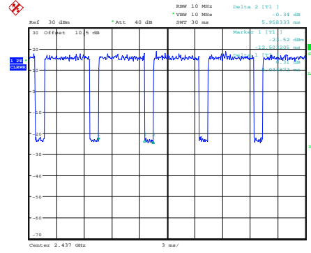
n40_2437MHz
