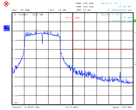
n40_2452MHz
