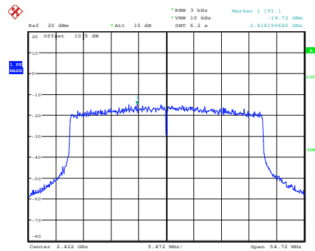
ax40_2422MHz
