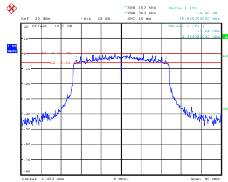
ax40_2452MHz
