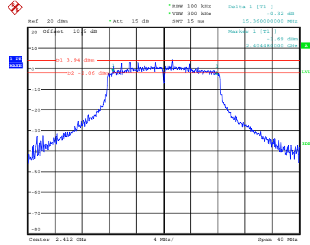
g_2412MHz
