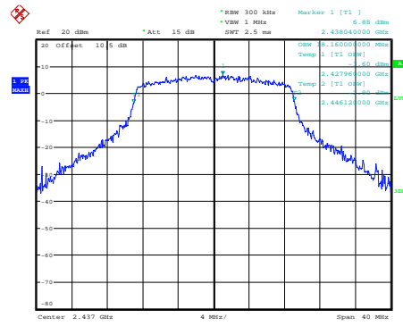
n20_2437MHz
