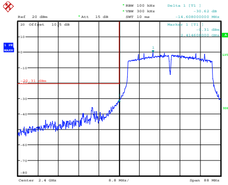
n40_2422MHz
