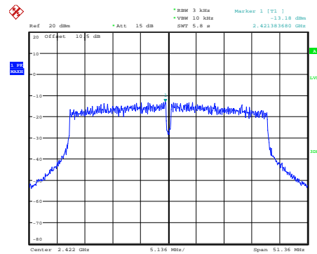
n40_2422MHz
