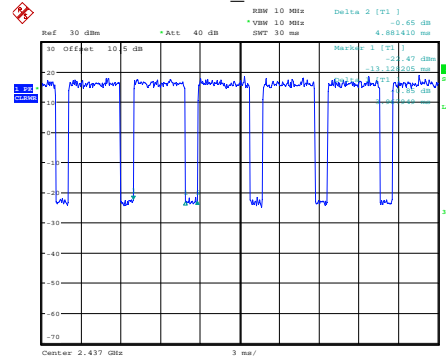
ax40_2437MHz
