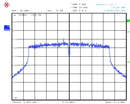
n40_2452MHz
