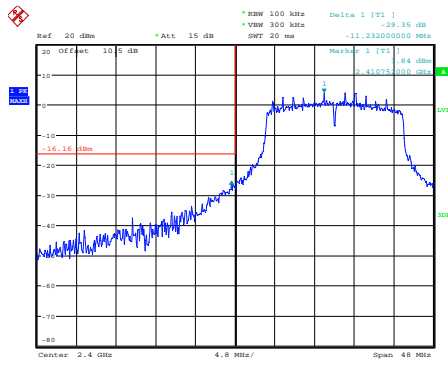
g_2412MHz
