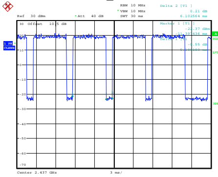
n20_2437MHz
