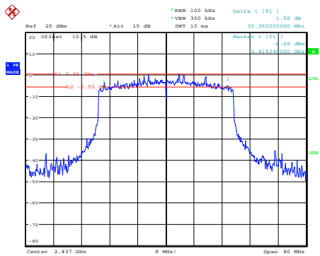
ax40_2437MHz
