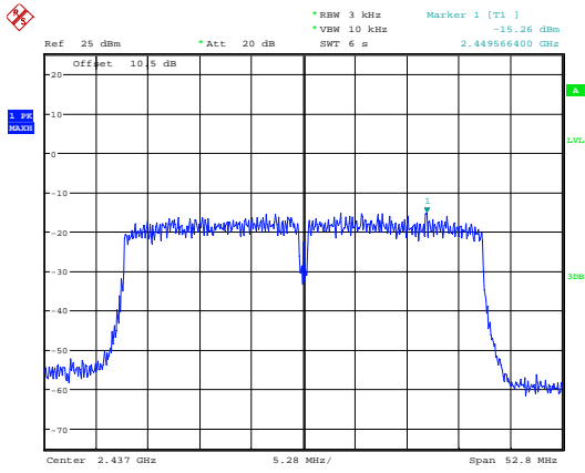
n40_2437MHz
