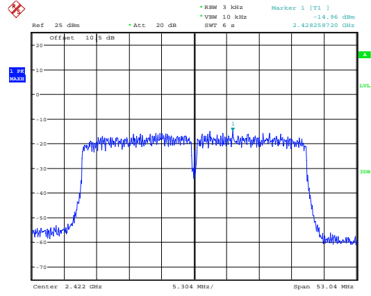
n40_2422MHz
