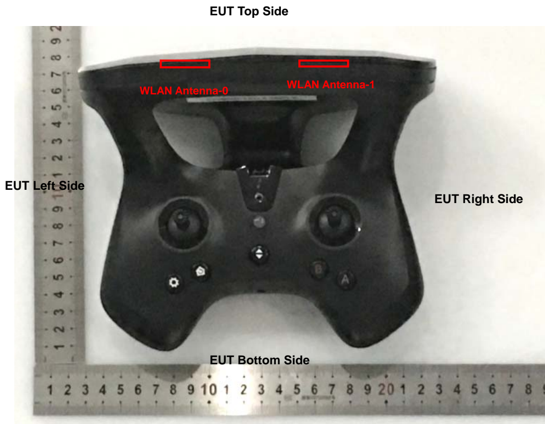
<EUT Front View>
