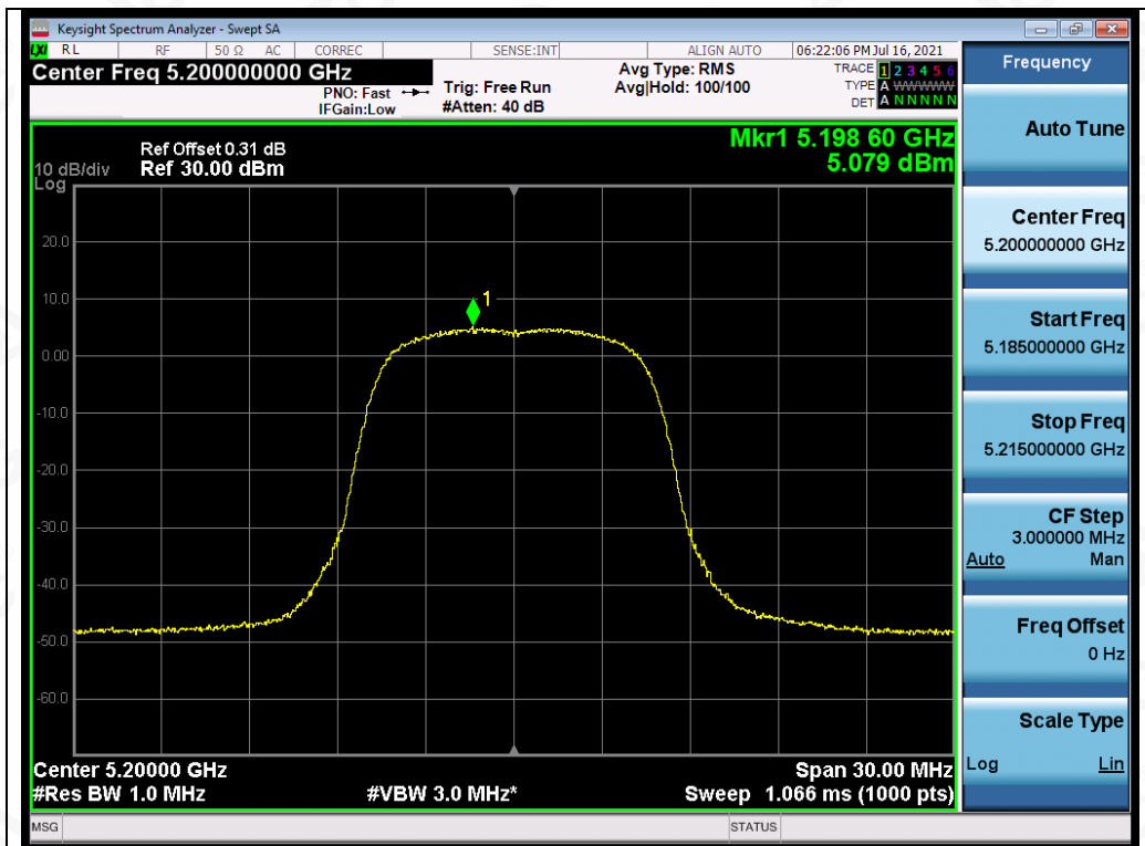
Test_Graph_OFDM_ANT2_5200_MCS0_PSD
