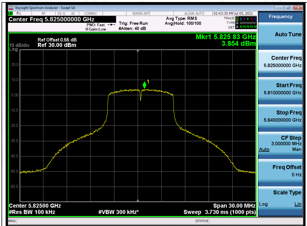
Test_Graph_OFDM_ANT1_5825_6Mbps_PSD
