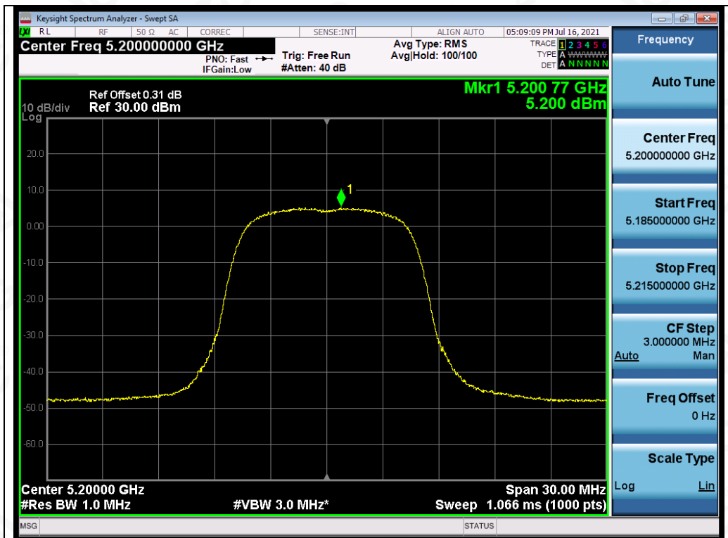
Test_Graph_OFDM_ANT1_5200_MCS0_PSD
