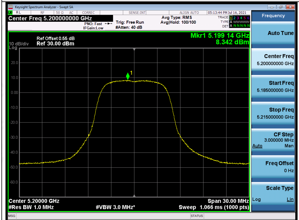
Test_Graph_OFDM_ANT1_5200_6Mbps_PSD
