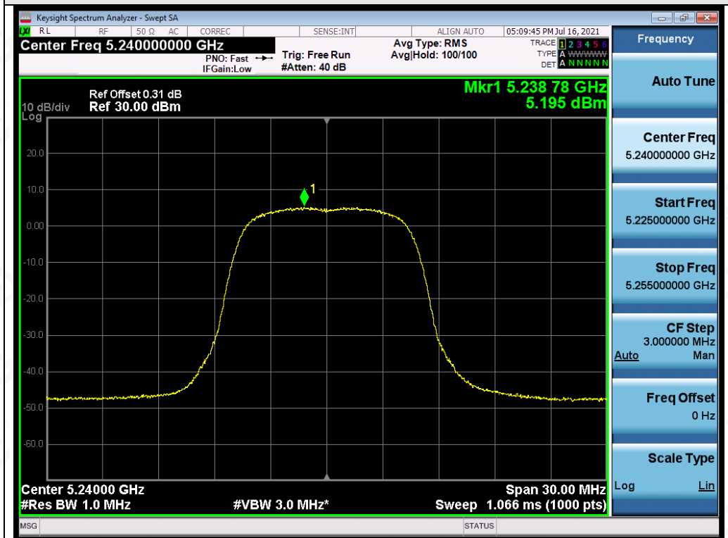
Test_Graph_OFDM_ANT1_5240_MCS0_PSD
