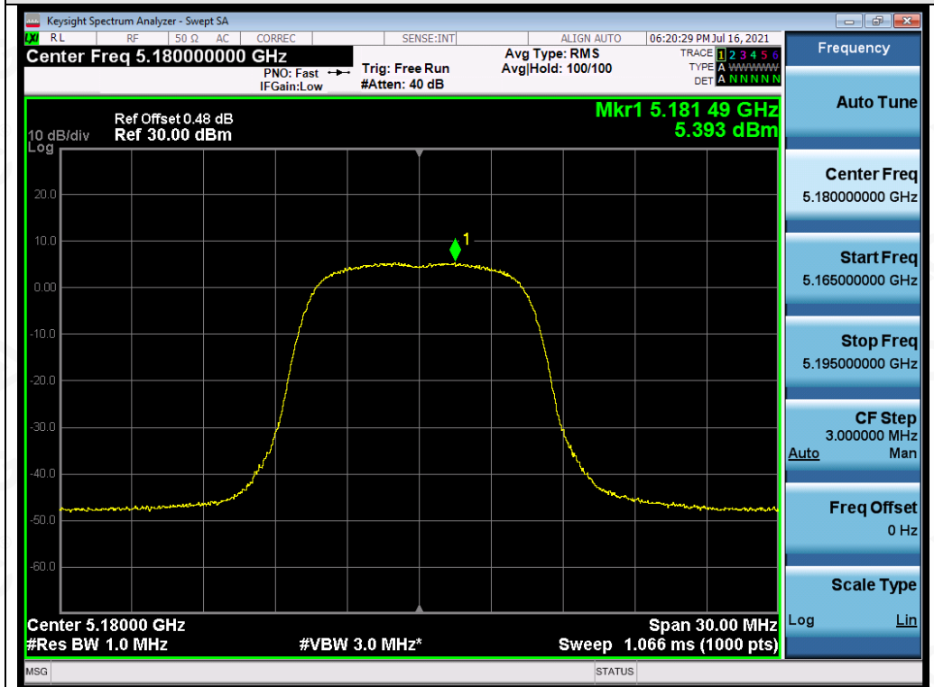
Test_Graph_OFDM_ANT2_5180_MCS0_PSD
