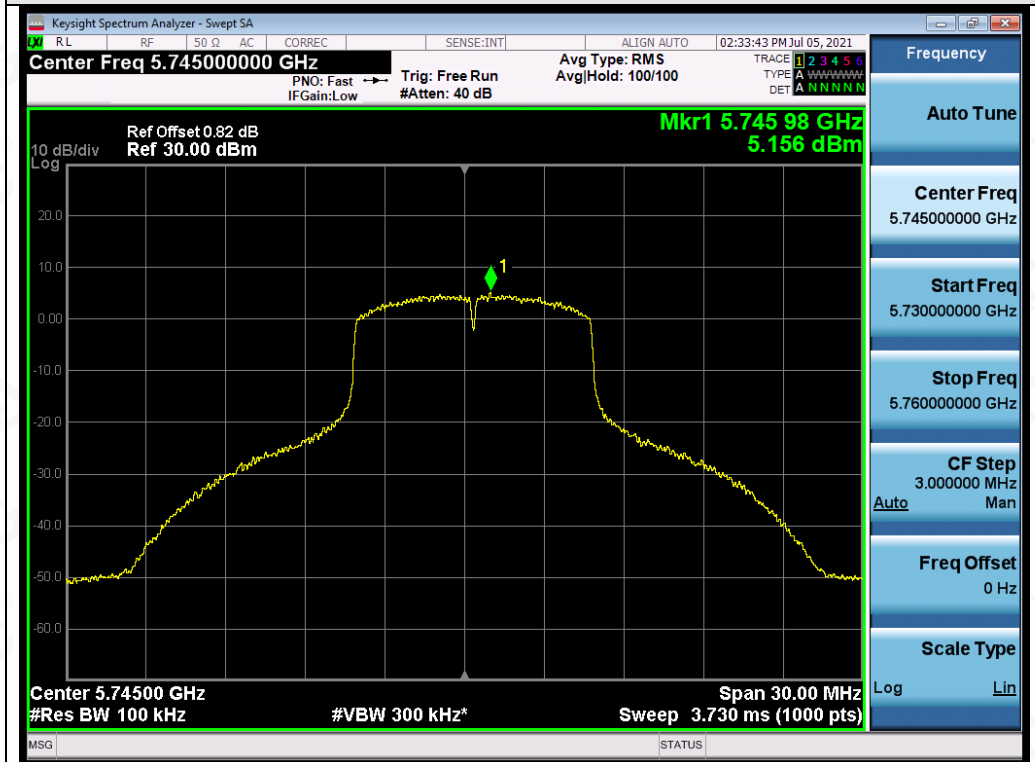
Test_Graph_OFDM_ANT1_5745_MCS0_PSD
