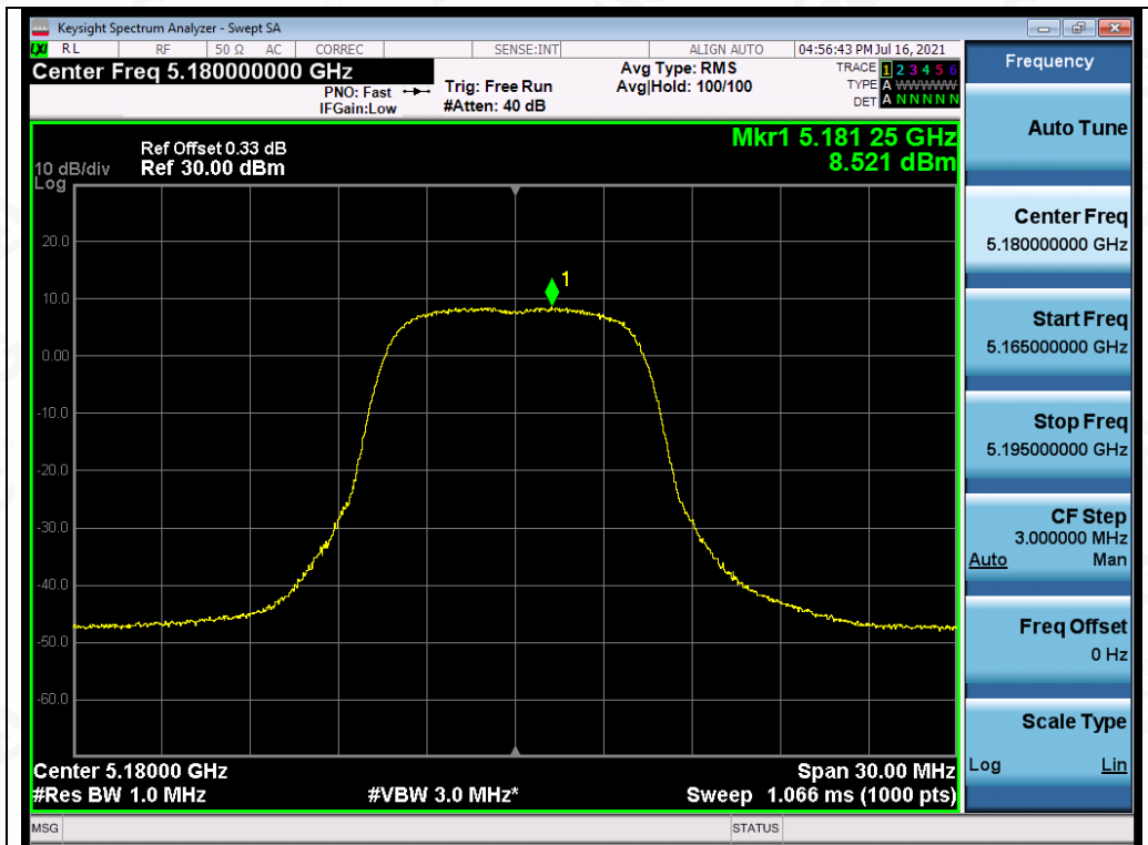
Test_Graph_OFDM_ANT1_5180_6Mbps_PSD
