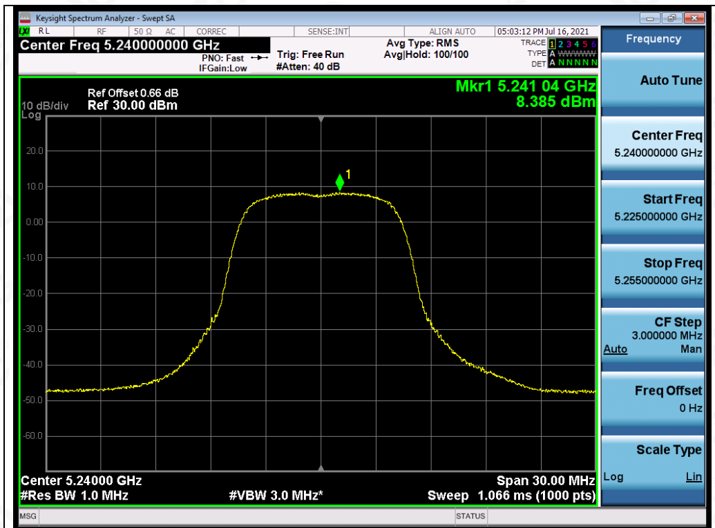
Test_Graph_OFDM_ANT1_5240_6Mbps_PSD
