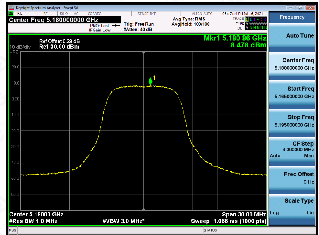
Test_Graph_OFDM_ANT2_5180_6Mbps_PSD
