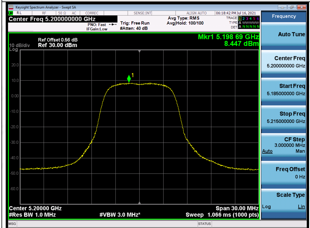
Test_Graph_OFDM_ANT2_5200_6Mbps_PSD
