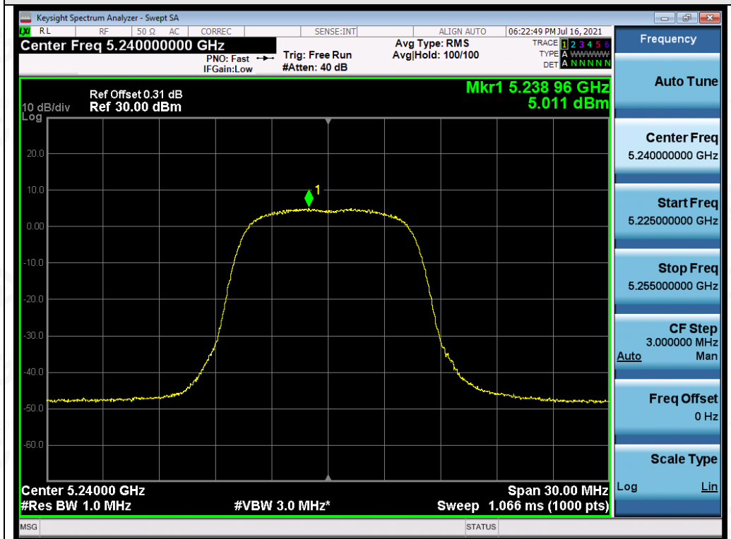
Test_Graph_OFDM_ANT2_5240_MCS0_PSD
