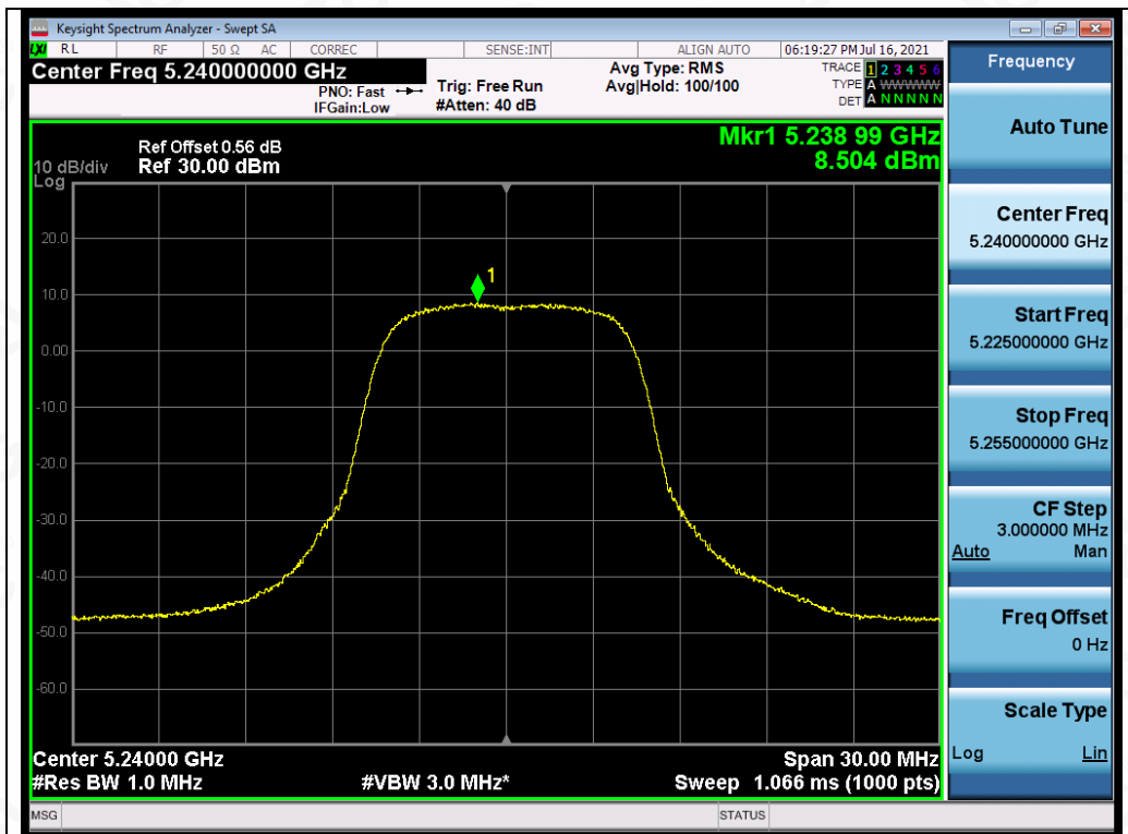
Test_Graph_OFDM_ANT2_5240_6Mbps_PSD
