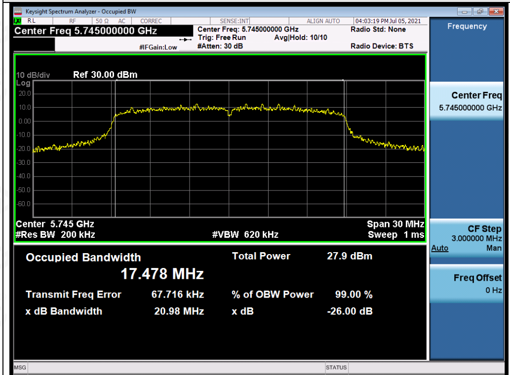
Test_Graph_802.11n20_ANT2_5745_MCS0_OBW
