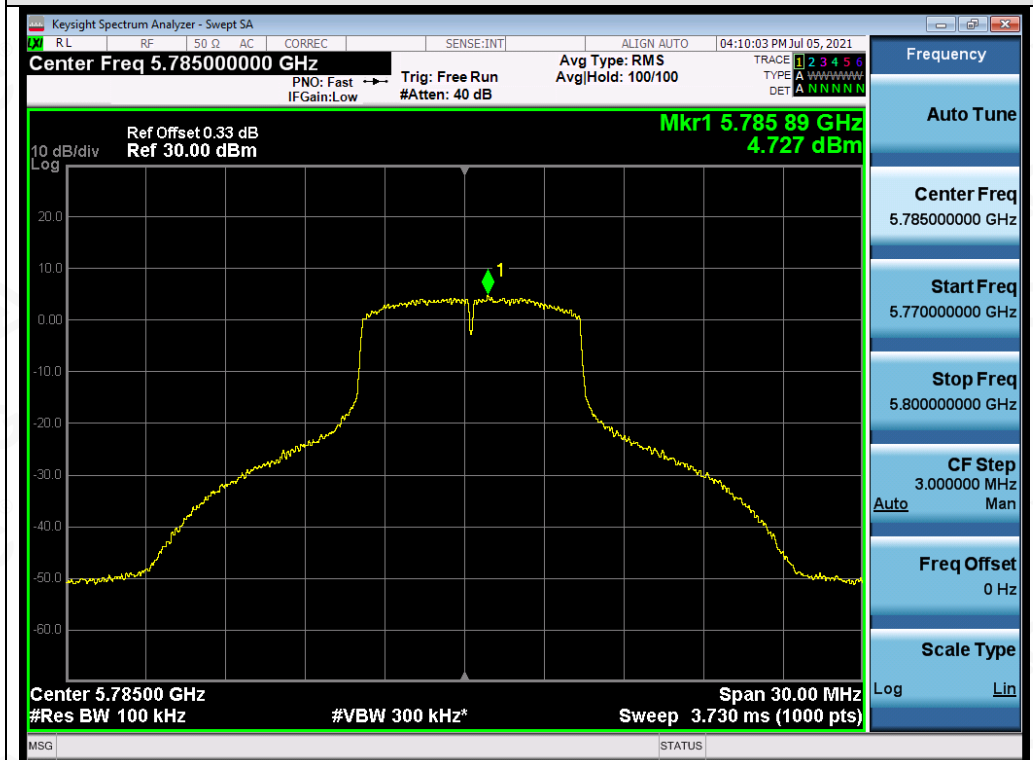
Test_Graph_OFDM_ANT2_5785_6Mbps_PSD
