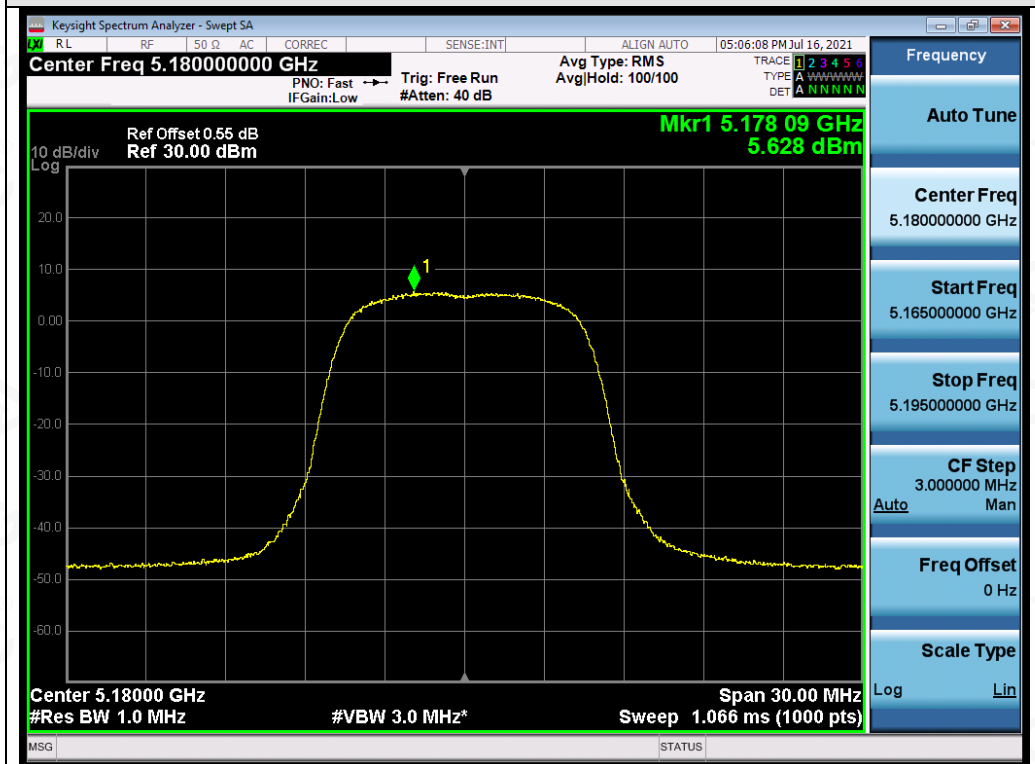
Test_Graph_OFDM_ANT1_5180_MCS0_PSD
