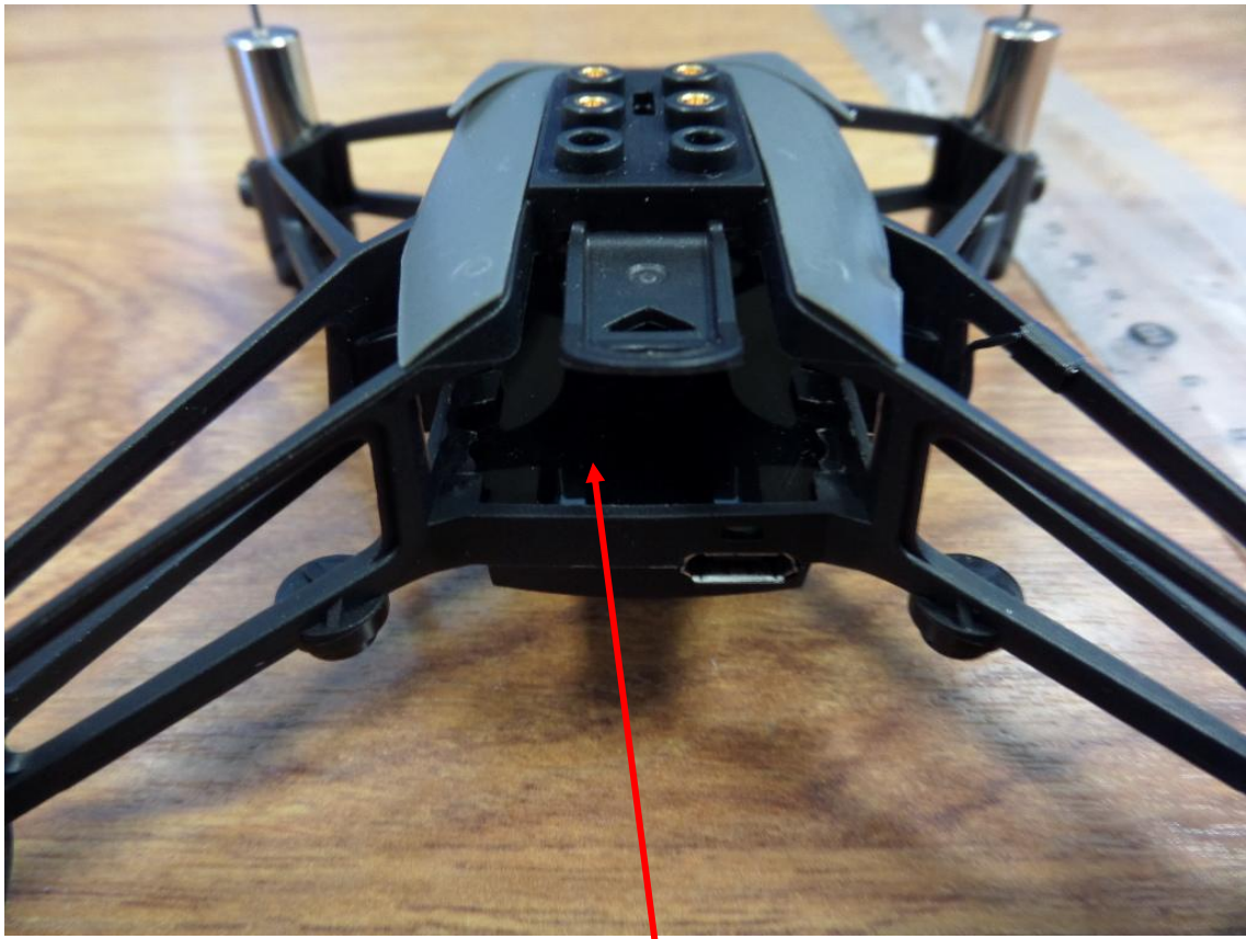
Label placement
