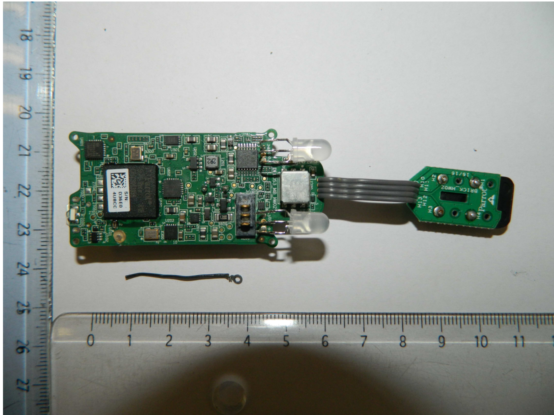
Mother Board (Bottom) without RF antenna
