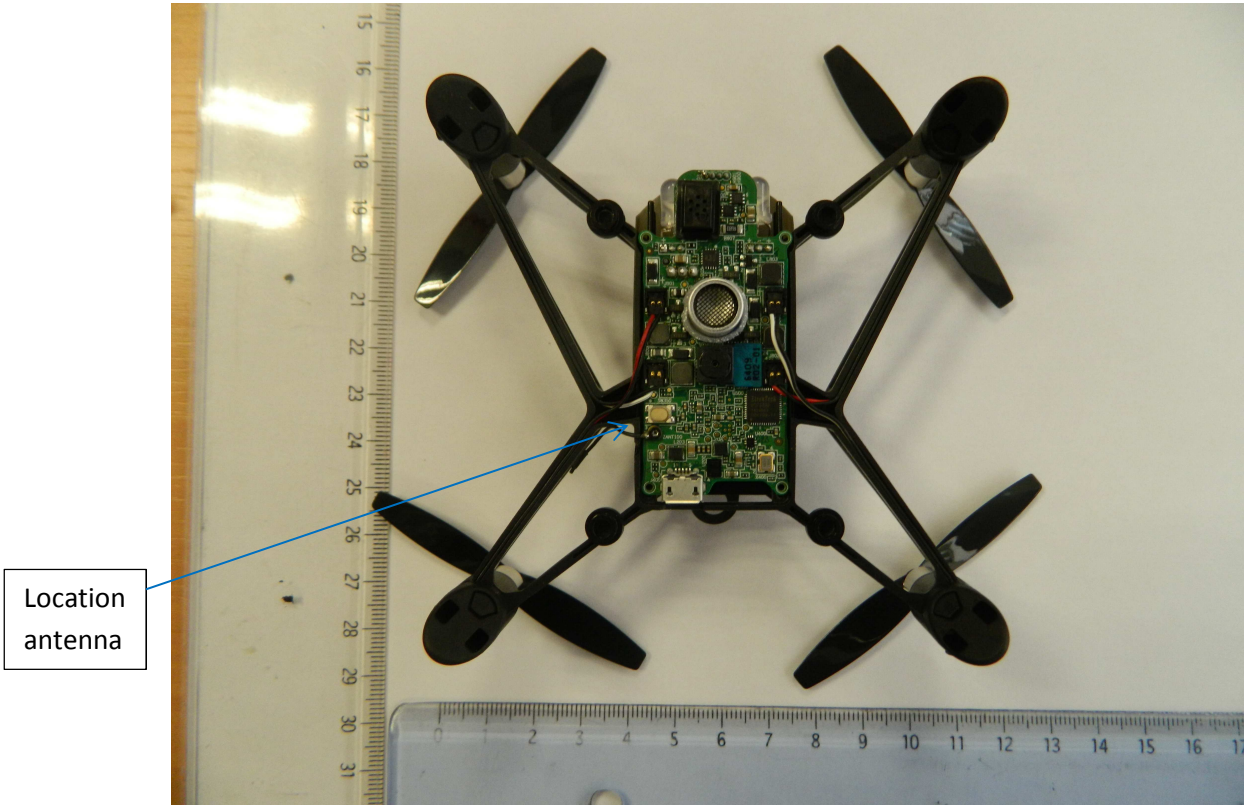
Mother Board (Top) with RF antenna
