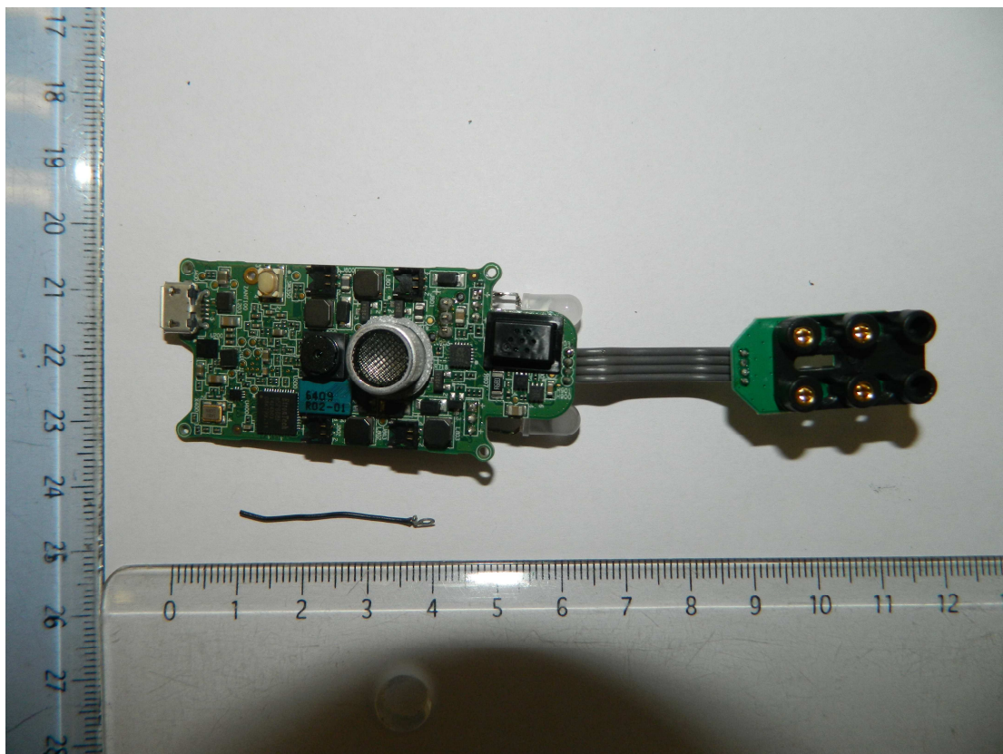
Mother Board (Top) without RF antenna
