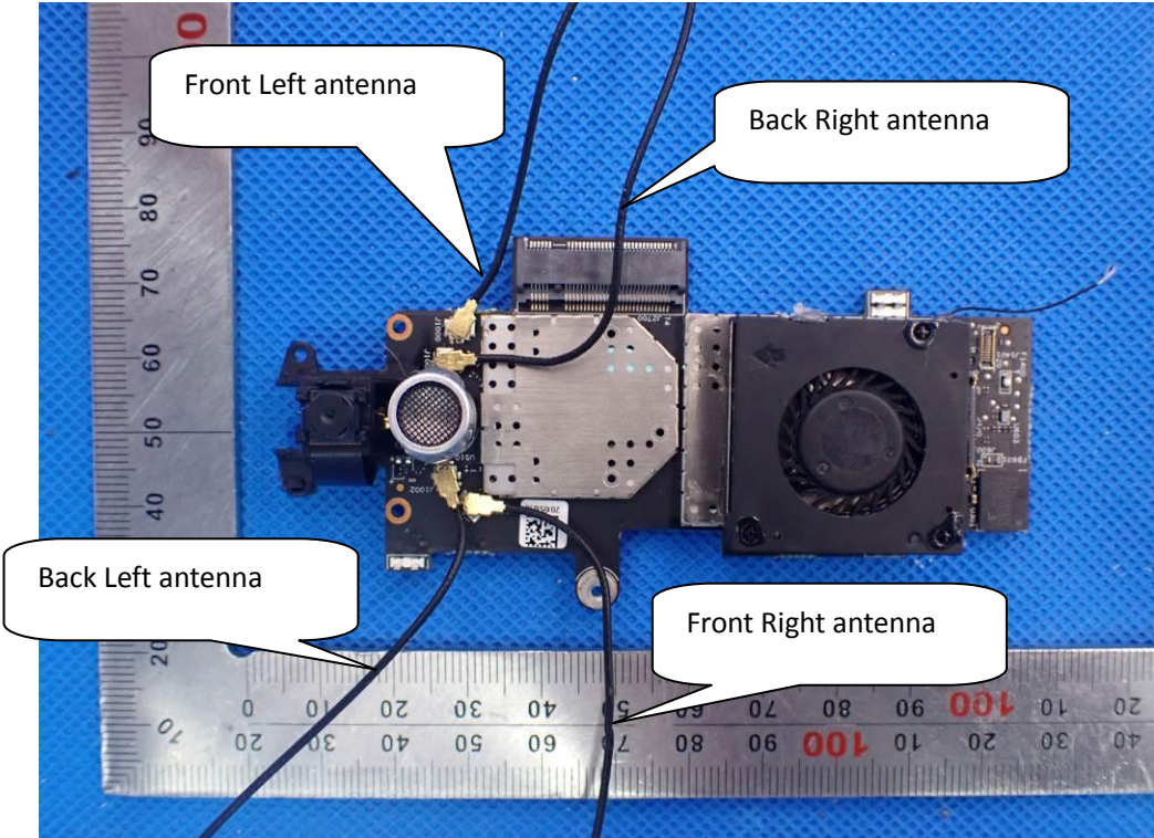
INTERNAL VIEW-20 OF EUT
