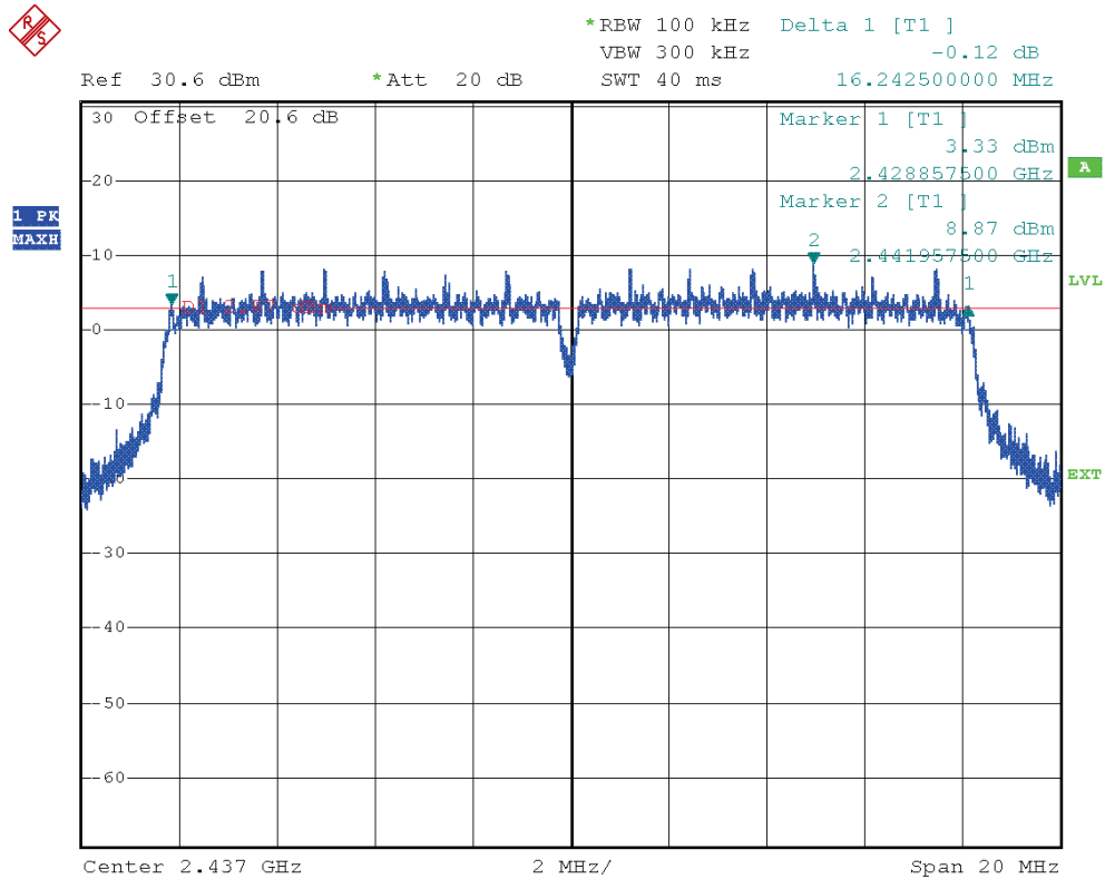
Channel 6 (F = 2437 MHz) – Mode 802.11g – bandwidth 20 MHz – Back Right
