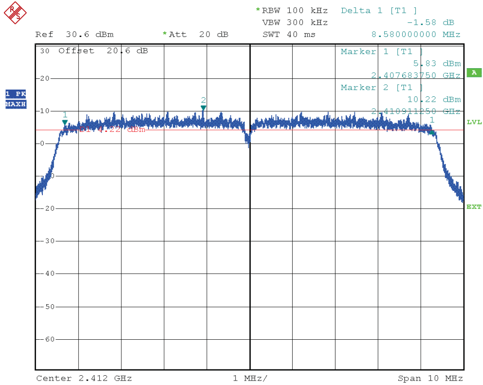
Channel 1 (F = 2412 MHz) – Mode 802.11n – bandwidth 10 MHz – Back Left
