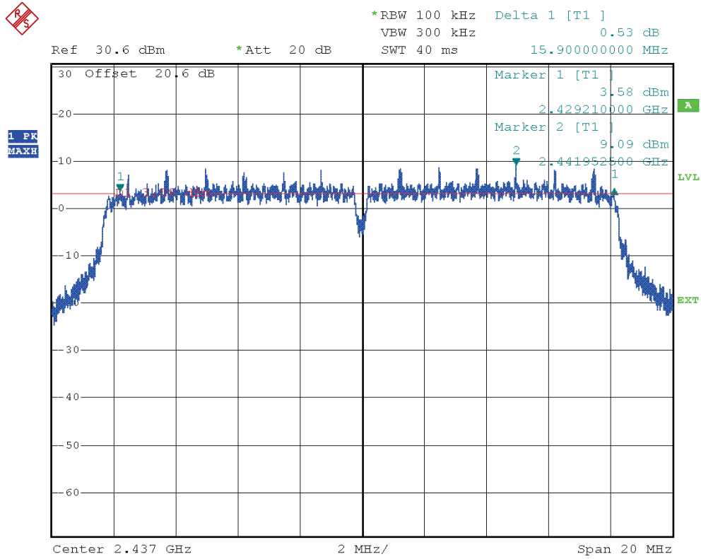
Channel 6 (F = 2437 MHz) – Mode 802.11g – bandwidth 20 MHz – Back Left
