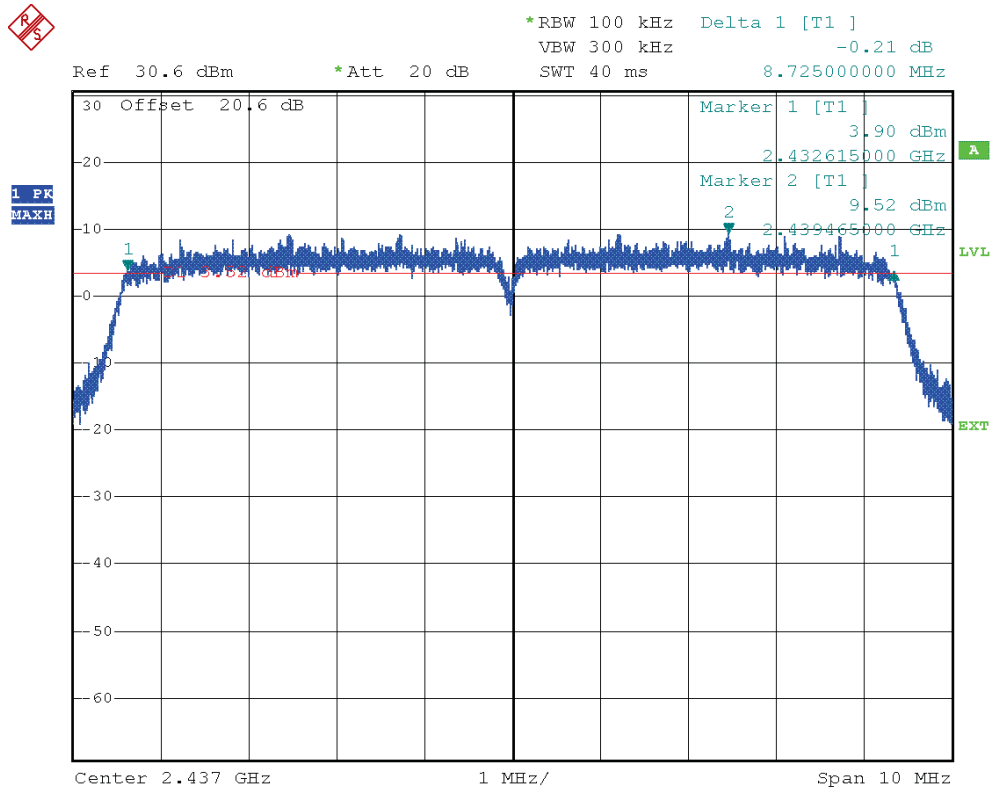
Channel 6 (F = 2437 MHz) – Mode 802.11n – bandwidth 10 MHz – Back Right
