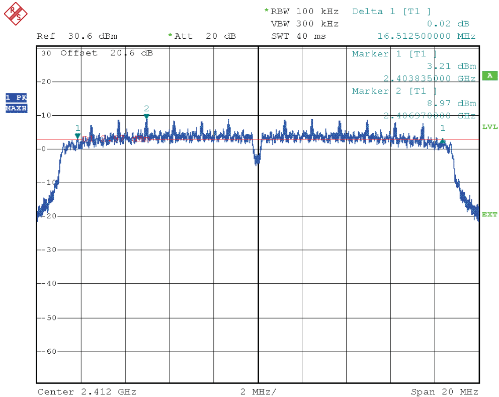
Channel 1 (F = 2412 MHz) – Mode 802.11n – bandwidth 20 MHz – Back Right
