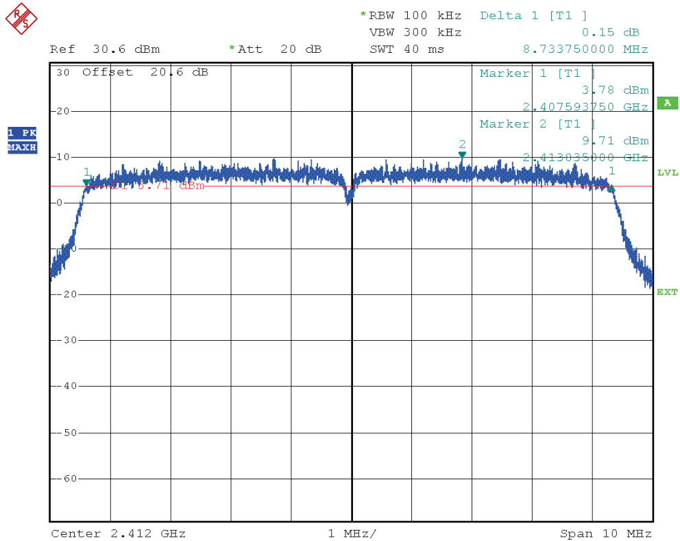
Channel 1 (F = 2412 MHz) – Mode 802.11n – bandwidth 10 MHz – Back Right
