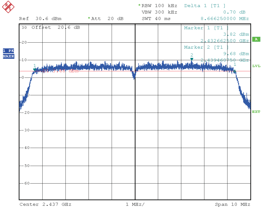
Channel 6 (F = 2437 MHz) – Mode 802.11n – bandwidth 10 MHz – Back Left
