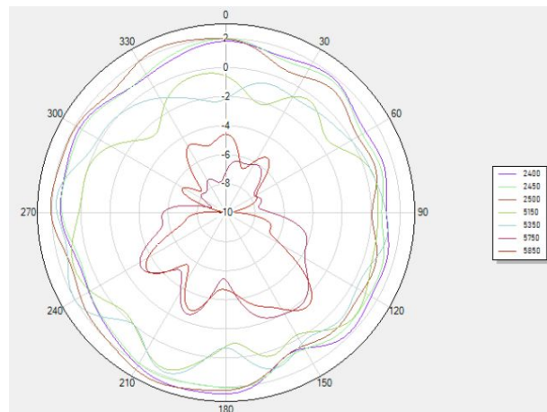
Theta 90 2D
