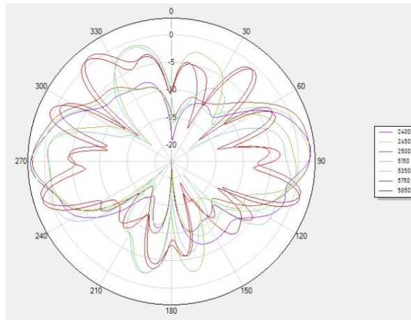
Phi 0 2D
