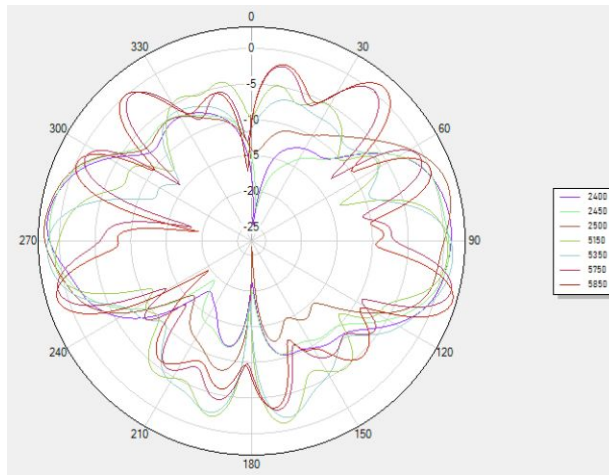
Phi 90 2D
