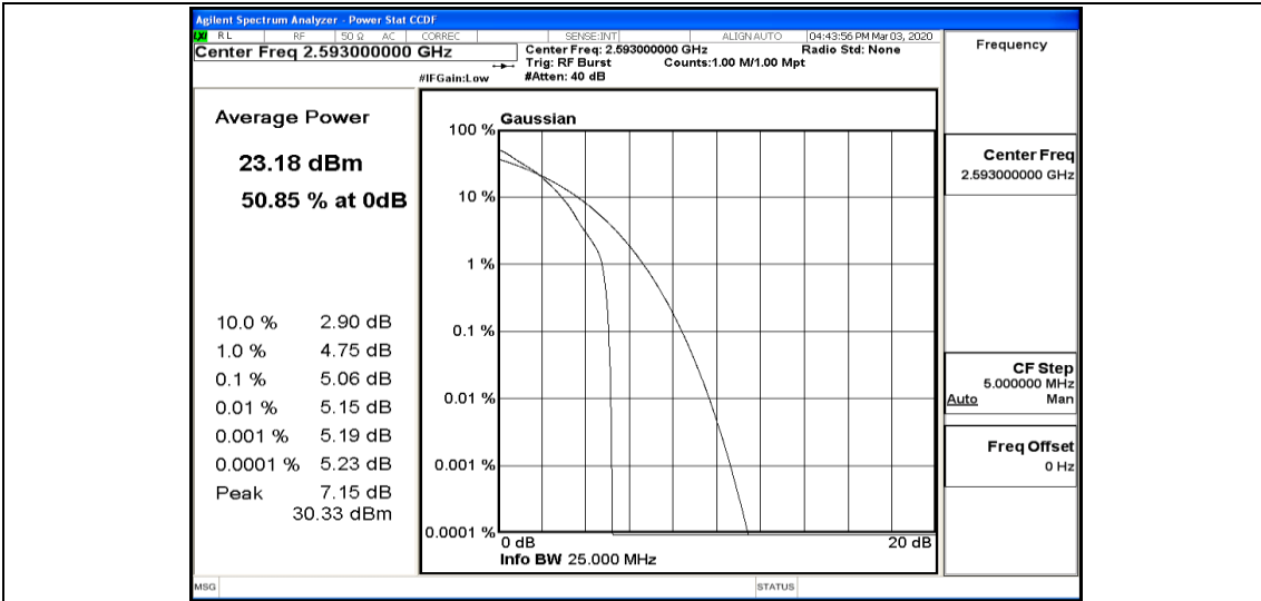
Band41-10MHz-QPSK-40620-50RB#0
