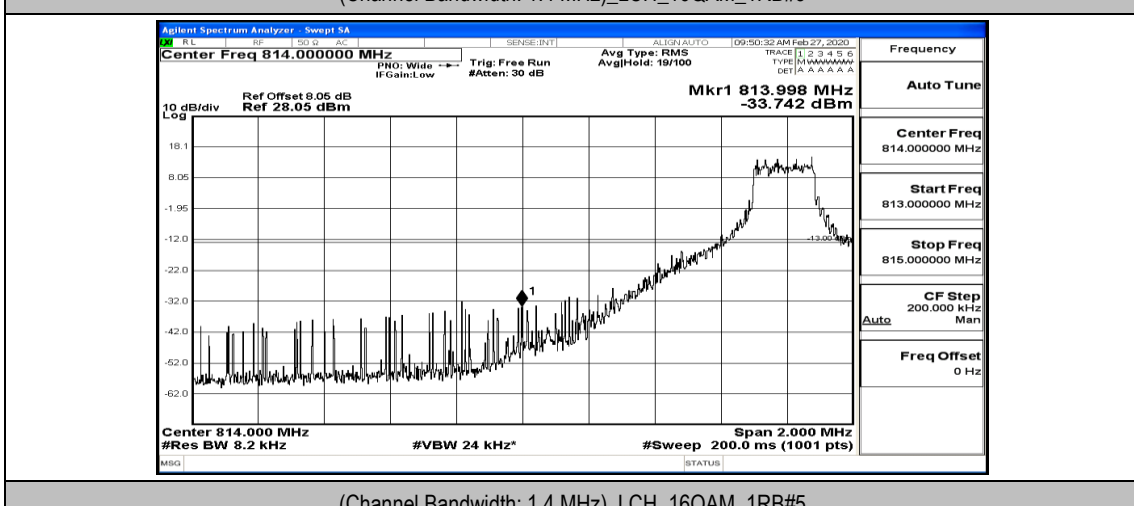
(Channel Bandwidth: 1.4 MHz)_LCH_16QAM_1RB#5
