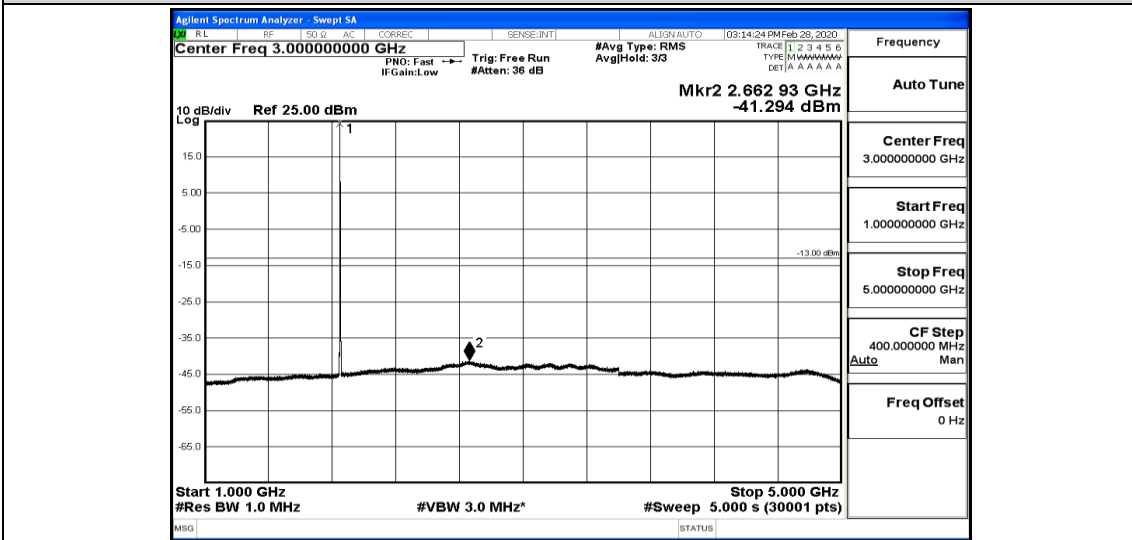
Band25-3MHz-16QAM-26055-1RB#0-Range5:5000~12000MHz
