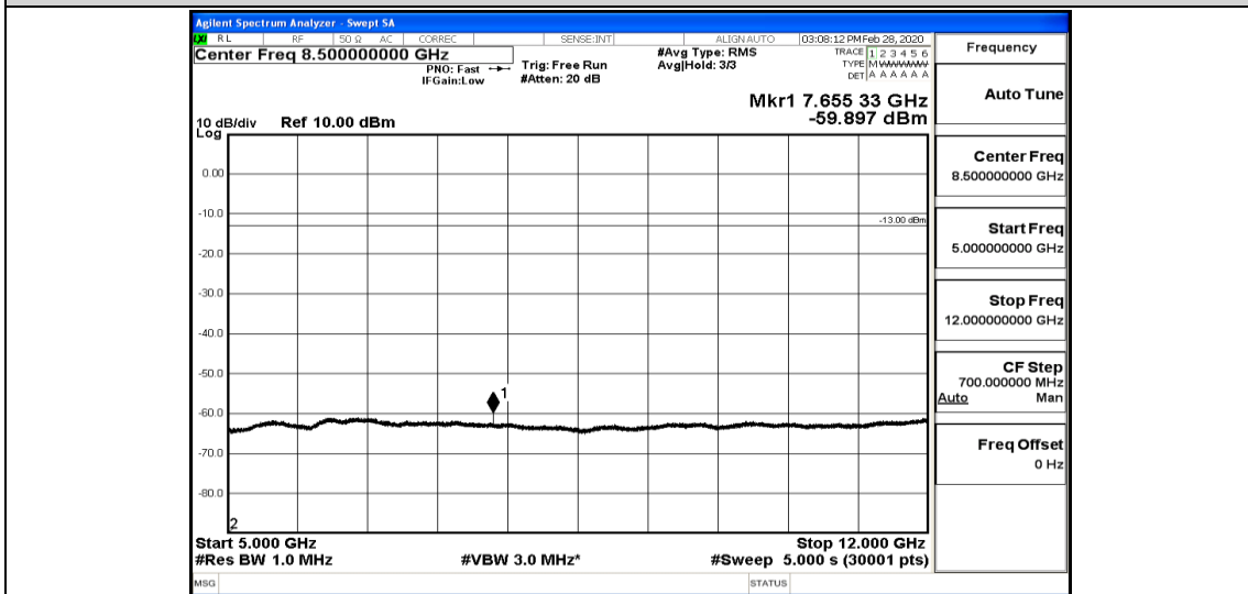
Band25-1.4MHz-16QAM-26683-1RB#0-Range6:12000~26500MHz
