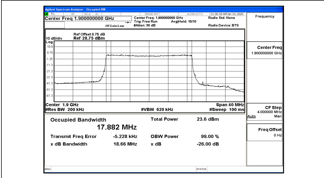
(Channel Bandwidth:20 MHz)_HCH_16QAM_100RB#0
