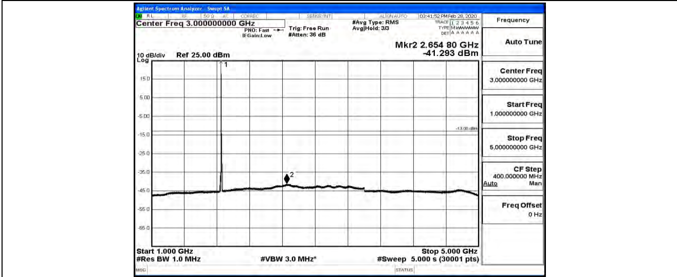
Band25-10MHz-QPSK-26090-1RB#0-Range5:5000~12000MHz
