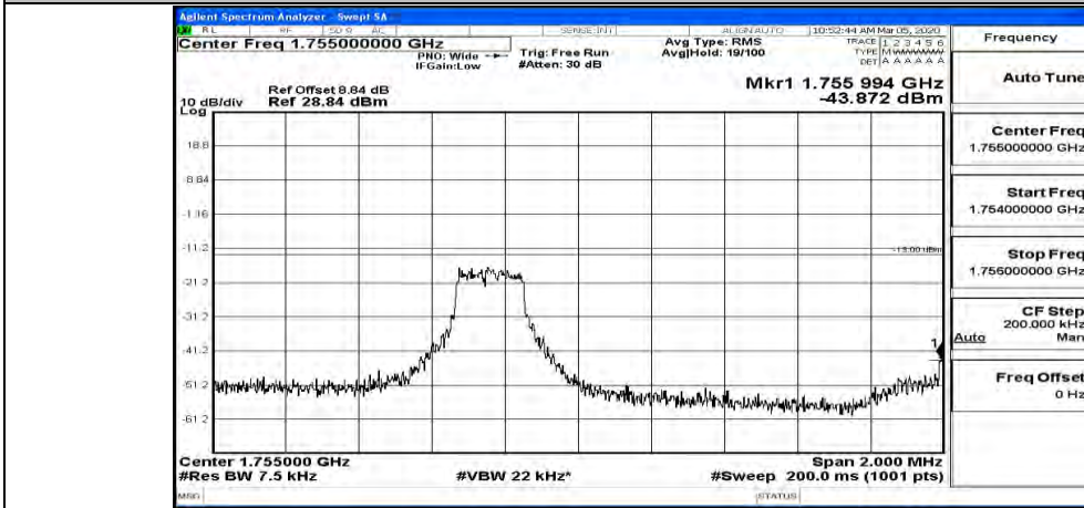
(Channel Bandwidth: 3 MHz)_HCH_QPSK_1RB#7
