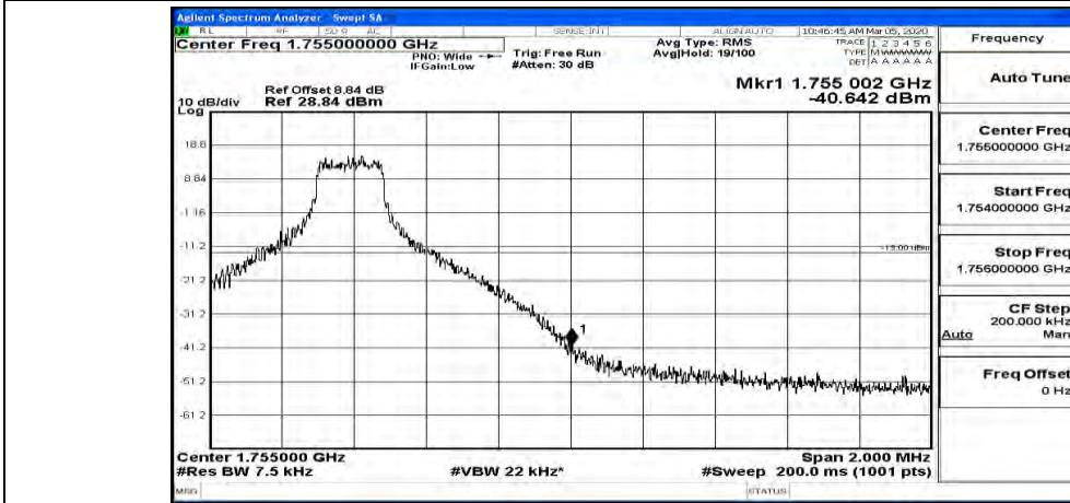
(Channel Bandwidth: 1.4 MHz)_HCH_16QAM_1RB#5
