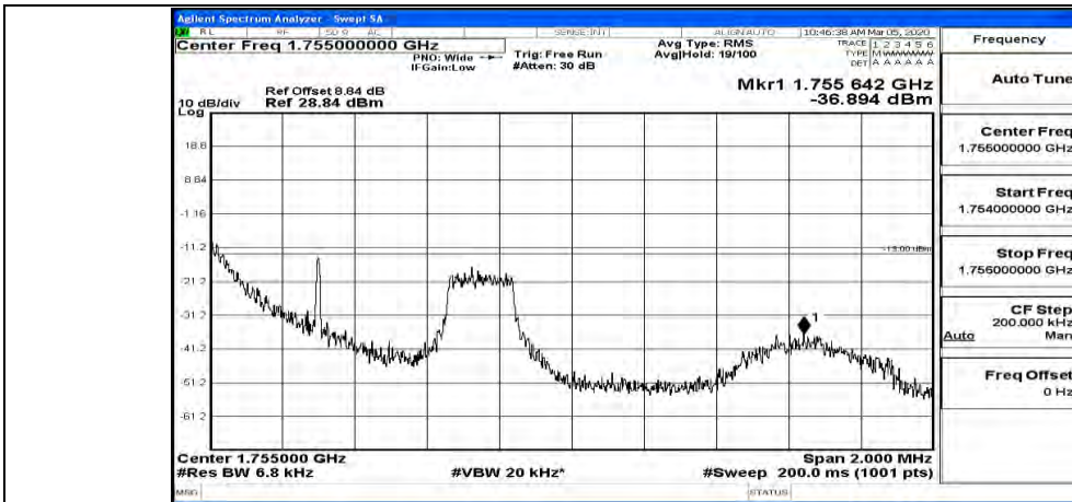
(Channel Bandwidth: 1.4 MHz)_HCH_16QAM_1RB#3
