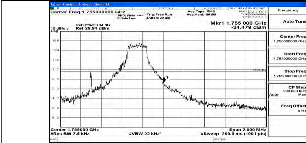
(Channel Bandwidth: 1.4 MHz)_HCH_16QAM_3RB#0
