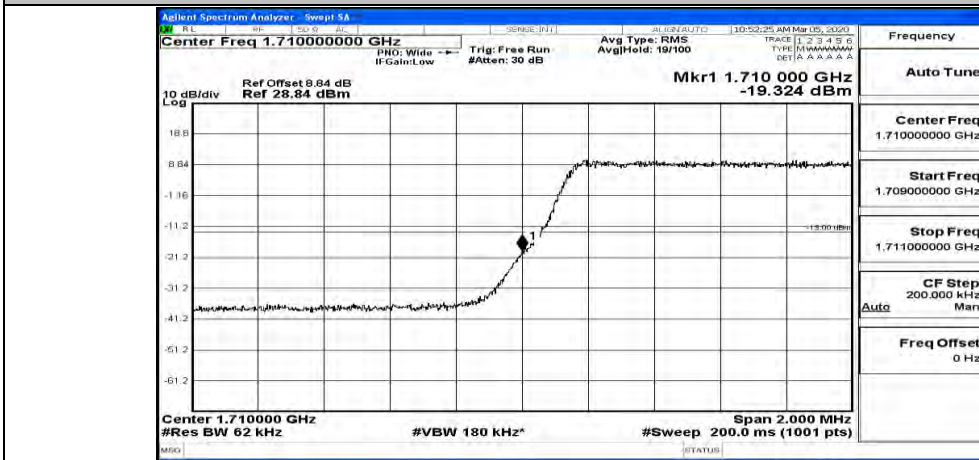
(Channel Bandwidth: 3 MHz)_LCH_QPSK_15RB#0
