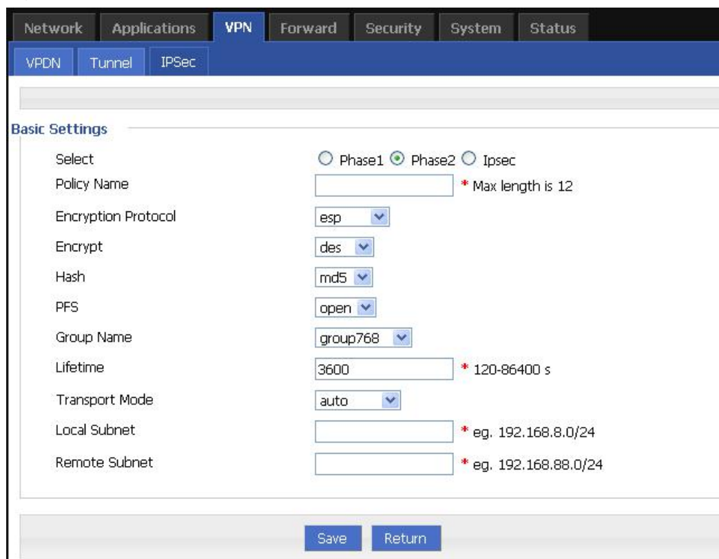
Figure 5-62 IPsec phase 2 configuration
