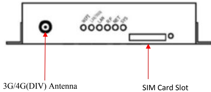
Figure 2-4 Front pannel
