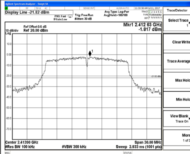
2397 MHz – 2427 MHz
