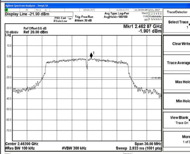
2447 MHz – 2477 MHz
