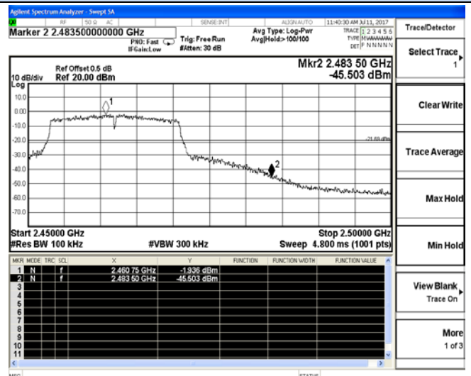
Channel 11 / 2462 MHz
