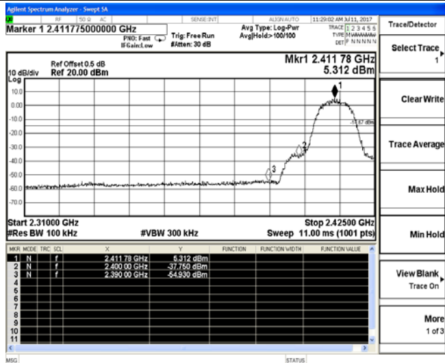
Channel 1 / 2412 MHz
