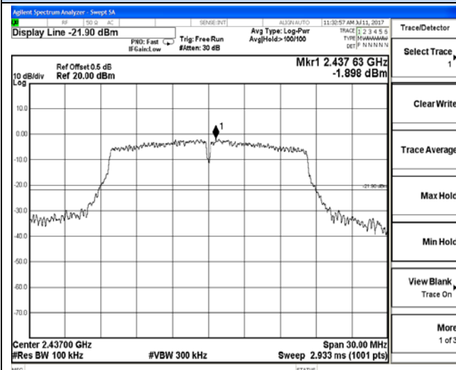
2422 MHz – 2452 MHz
