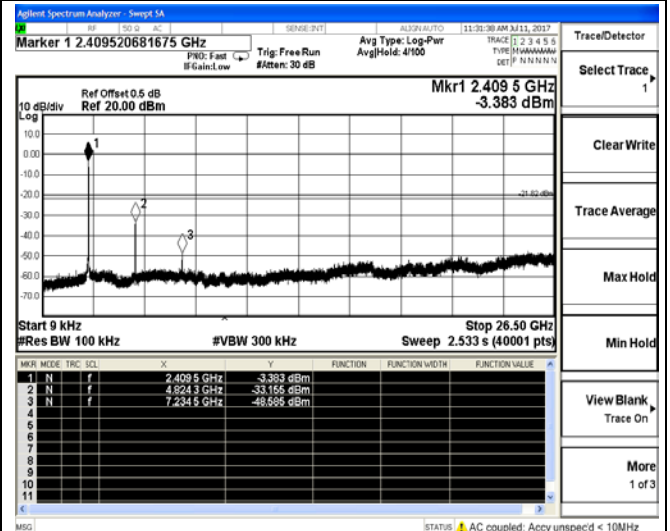
9 KHz – 26.5 GHz
