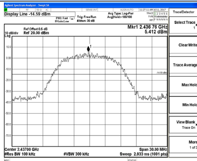
2422 MHz – 2452 MHz
