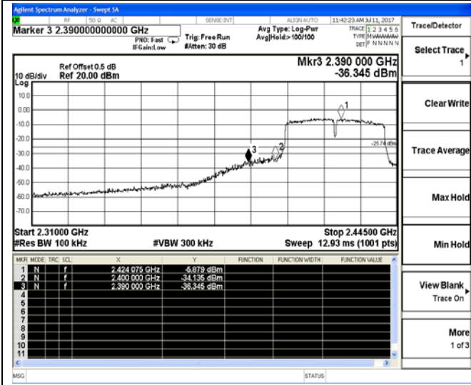
Channel 3 / 2422 MHz
