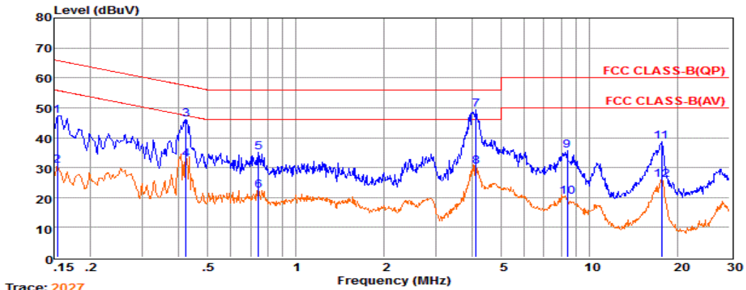
Trace: 2027
