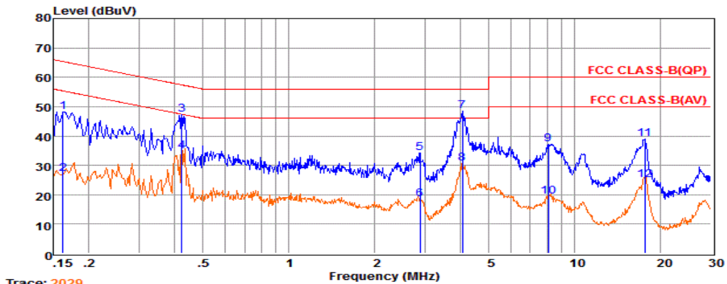
Trace: 2029
