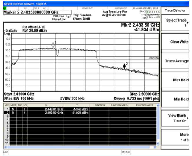
Channel 9 / 2452 MHz
