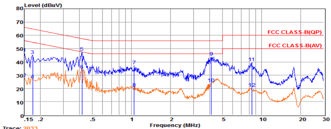
Trace: 2033
