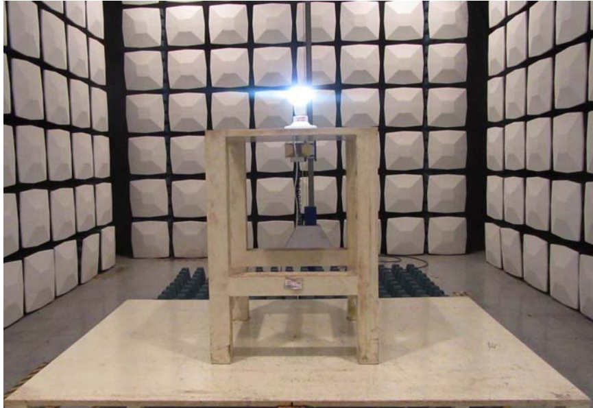
Radiated Disturbance Test Setup Rear View (Above 1GHz)
