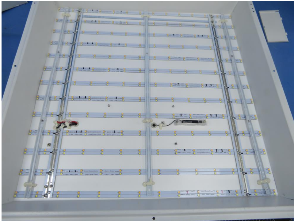
View of LED part of LE-LP40L6060Q01 (representative for all models)
