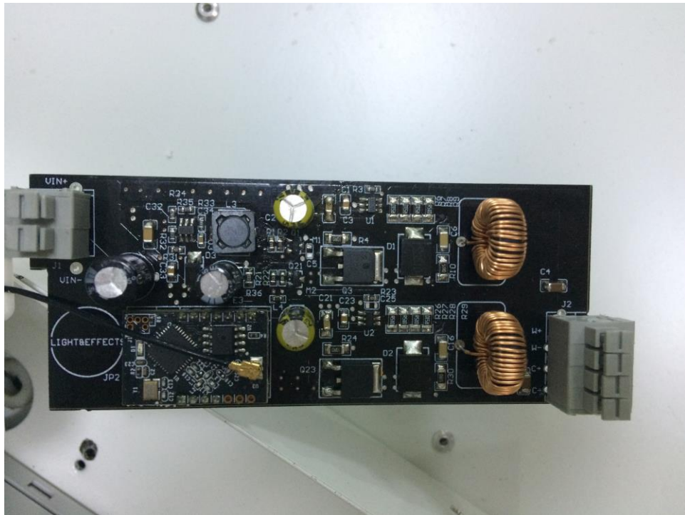
View of control circuit (representative for all models)
