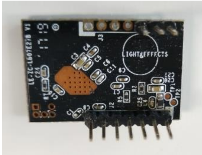
View of wireless module (representative for all models)
