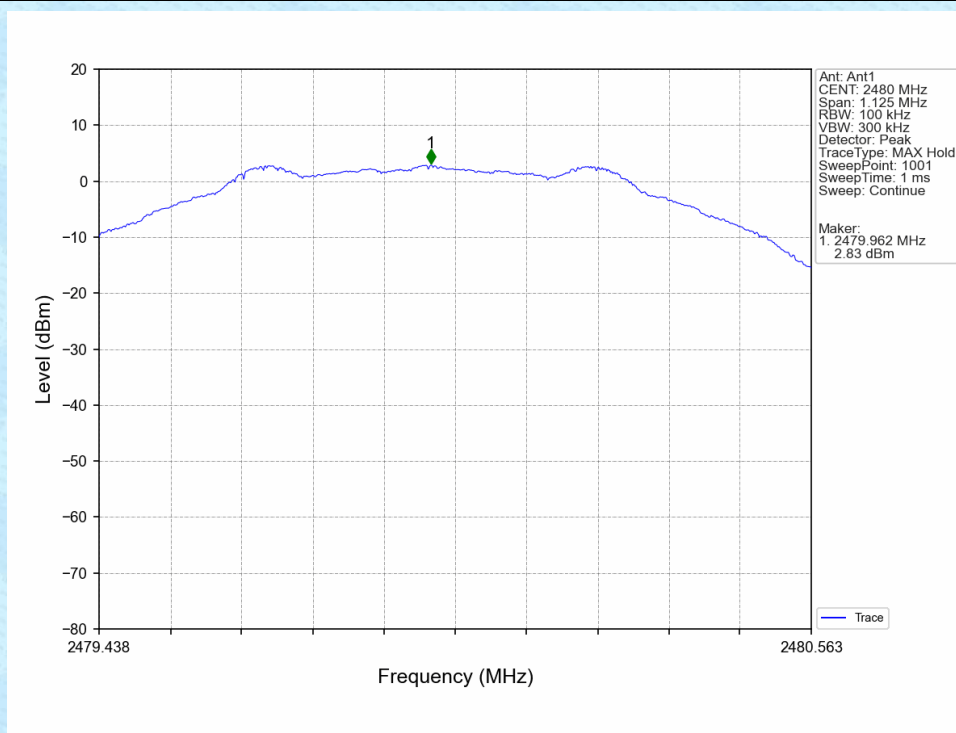
1M_HCH_2480MHz_Ant1_NTNV
