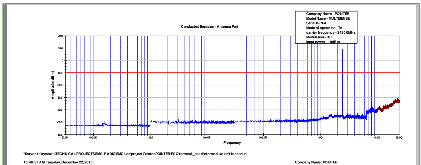
Figure 27 2480 MHz High*
